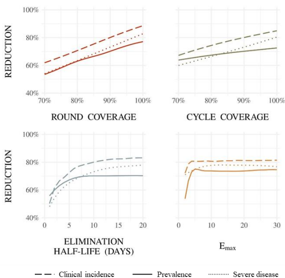
Figure A2.10: For SMC with dominant blood stage activity and initial, complete liver stage clearance, (A) illustrative Gaussian Process regression emulator predictions for the relationship between SMC properties and their direct effects on clinical incidence, prevalence, and severe disease reduction in children aged three to 59 months receiving SMC, and (B) illustrative Gaussian Process regression emulator predictions for the relationship between SMC properties and their indirect effects on clinical incidence, prevalence, and severe disease reduction in children aged 60 to 119 months not receiving SMC
