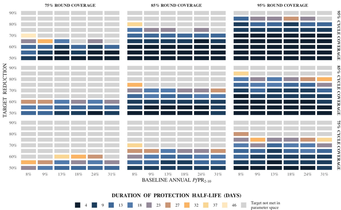
Figure 4: Summary of predicted minimum parameter values for SMC with dominant blood stage activity and initial, complete liver stage clearance to achieve target reductions in clinical incidence and severe disease
