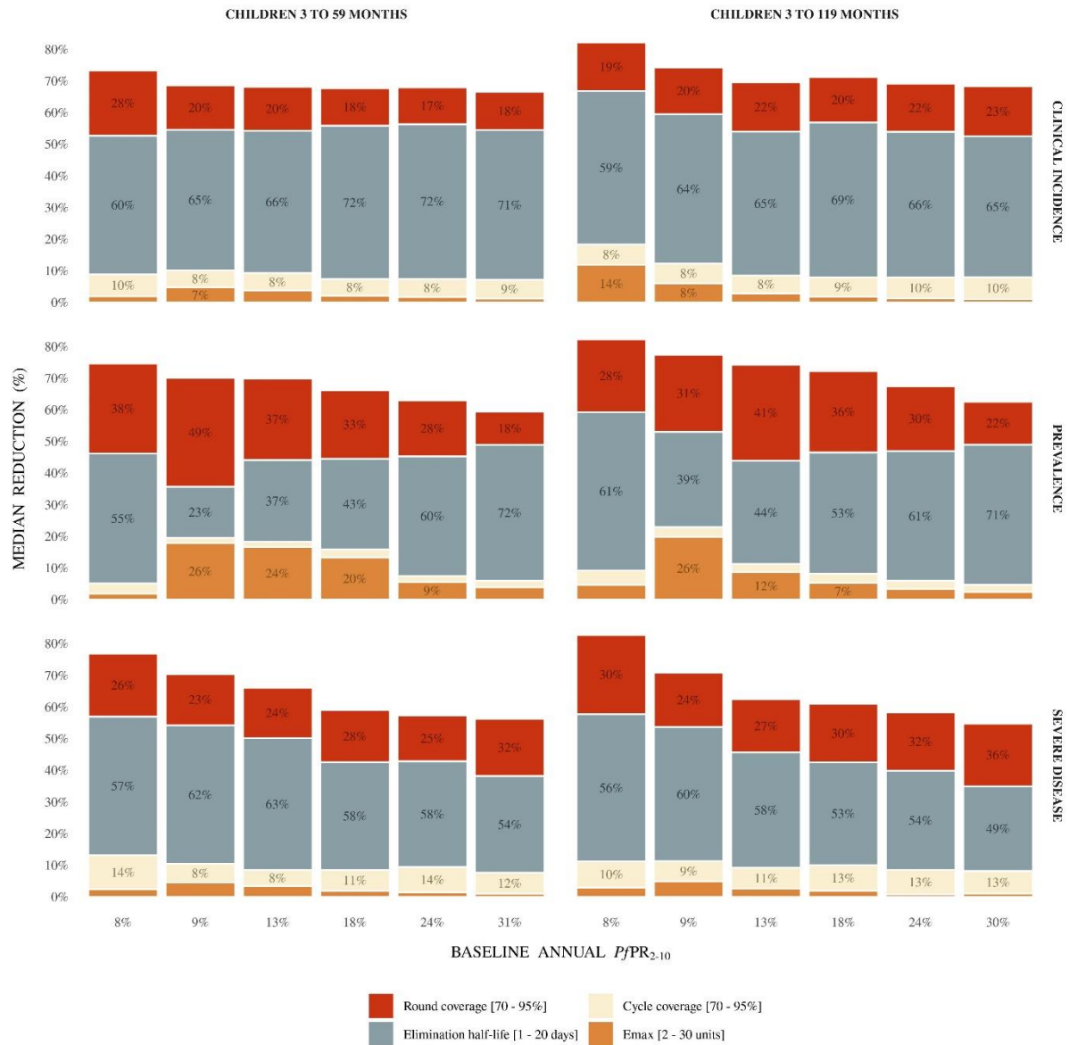
Figure A2.3: For SMC with blood stage activity only, drivers of impact on predicted levels of reduction of clinical incidence, prevalence, and severe disease in two scenarios – delivered to children aged three to 59 months or three to 119 months compared with the no intervention counterfactual
