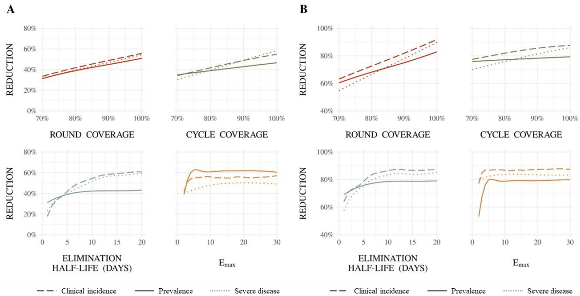
Figure A2.9: For SMC with dominant blood stage activity and initial, complete liver stage clearance, (A) illustrative Gaussian Process regression emulator predictions for the relationship between SMC properties and their direct effects on clinical incidence, prevalence, and severe disease reduction for a drug profile with low coverage and low protective efficacy, and (B) illustrative Gaussian Process regression emulator predictions for the relationship between SMC properties and their indirect effects on clinical incidence, prevalence, and severe disease reduction for a drug profile with high coverage and high protective efficacy
