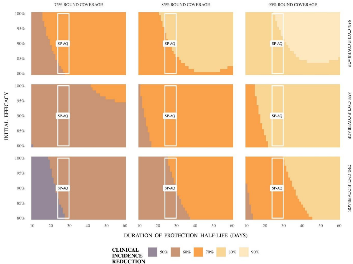
Figure A2.12: For SMC with dominant liver stage activity and initial, complete blood stage clearance, impact of a change in coverage on the predicted relative reduction in clinical incidence (measured over a four-month intervention period) following SMC compared with a no intervention counterfactual
