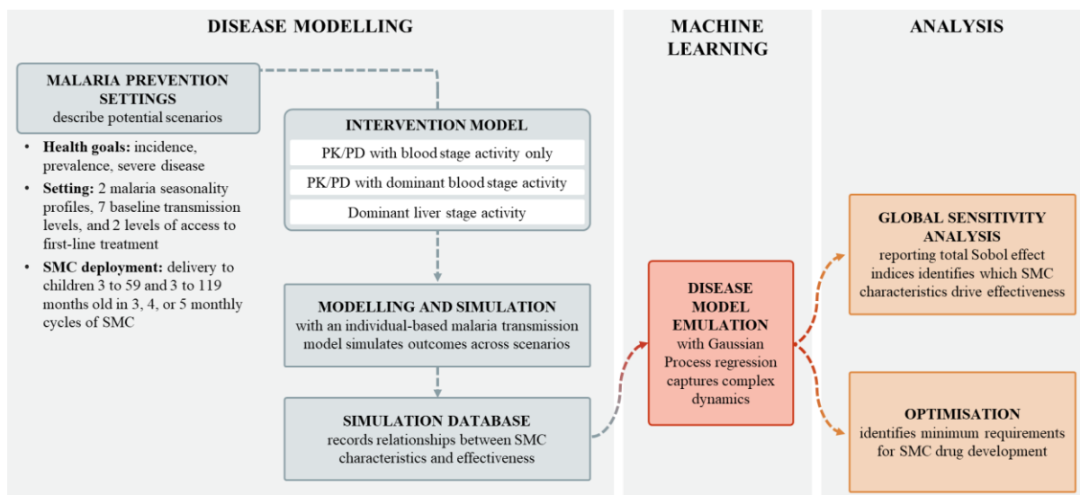
Figure A1.3: Evidence generation framework combining individual-based malaria transmission modelling with statistical methods to support the identification of minimum necessary SMC product characteristics
