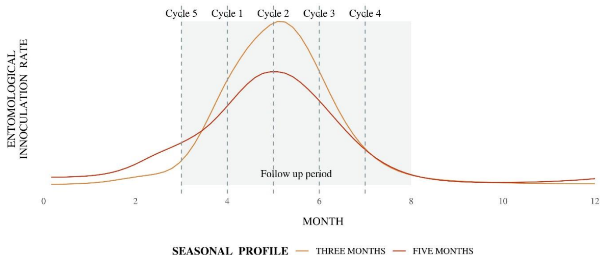
Figure A1.2: Seasonality profiles and SMC cycle timing
