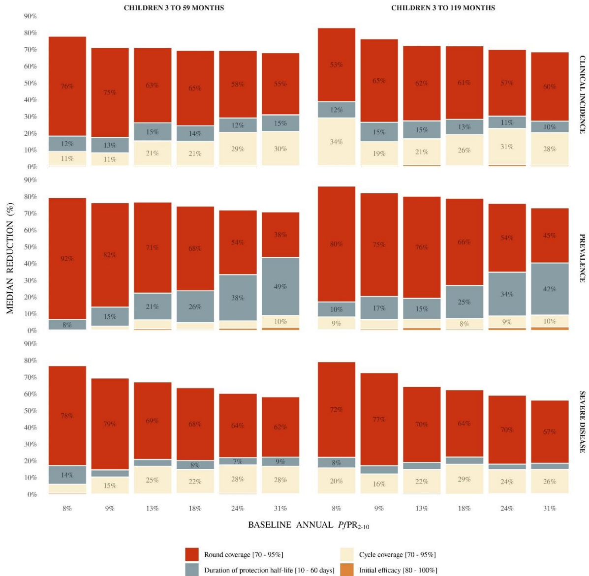
Figure A2.5: For SMC with dominant liver stage activity and initial, complete blood stage clearance, drivers of impact on predicted levels of reduction of clinical incidence, prevalence, and severe disease in two scenarios – delivered to children aged three to 59 months or three to 119 months compared with the no intervention counterfactual
