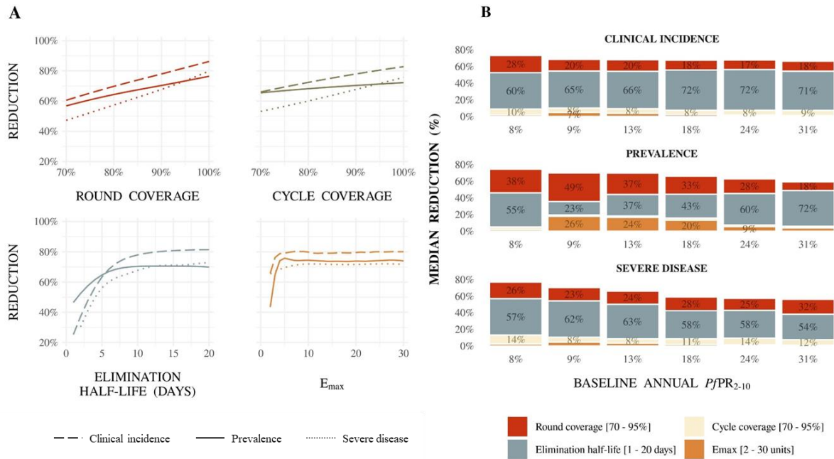
Figure A2.1: For SMC with blood stage activity only, (A) illustrative Gaussian Process regression emulator predictions for the relationship between SMC properties and clinical incidence, prevalence, and severe disease reduction, and (B) drivers of impact on predicted clinical incidence, prevalence, and severe disease reduction for SMC in children three to 59 months of age, compared with a no intervention counterfactual
