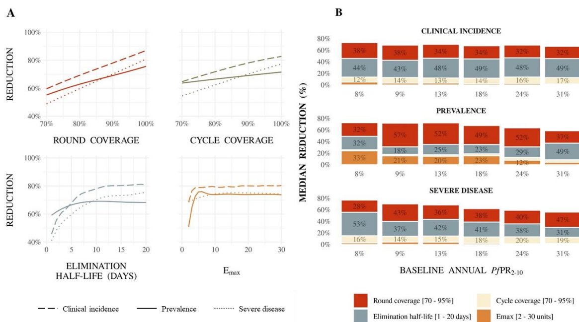
Figure 2: For SMC with dominant blood stage activity and initial, complete liver stage clearance, (A) illustrative Gaussian Process regression emulator predictions for the relationship between SMC properties and clinical incidence, prevalence, and severe disease reductions, and (B) drivers of impact on predicted clinical incidence, prevalence, and severe disease reduction for SMC in children three to 59 months of age, compared with a no intervention counterfactual
