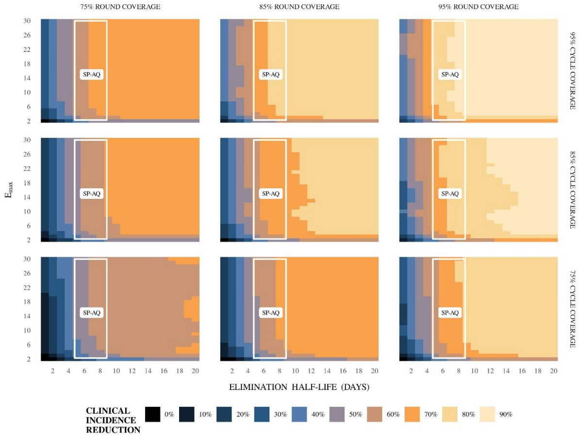
Figure A2.11: For SMC with blood stage activity only, impact of a change in coverage on the predicted relative reduction in clinical incidence (measured over a four-month intervention period) following SMC compared with a no intervention counterfactual
