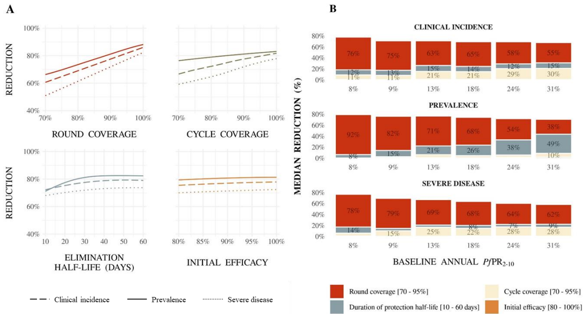
Figure A2.2: For SMC with dominant liver stage activity and initial, complete blood stage clearance, (A) illustrative Gaussian Process regression emulator predictions for the relationship between SMC properties and clinical incidence, prevalence, and severe disease reduction, and (B) drivers of impact on predicted clinical incidence, prevalence, and severe disease reduction for SMC in children three to 59 months of age, compared with a no intervention counterfactual
