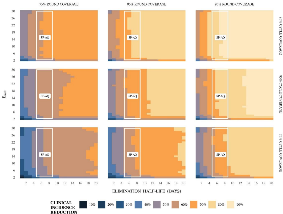
Figure 3: For SMC with dominant blood stage activity and initial, complete liver stage clearance, impact of a change in coverage on the predicted relative reduction in clinical incidence (measured over a four-month intervention period) following SMC compared with a no intervention counterfactual
