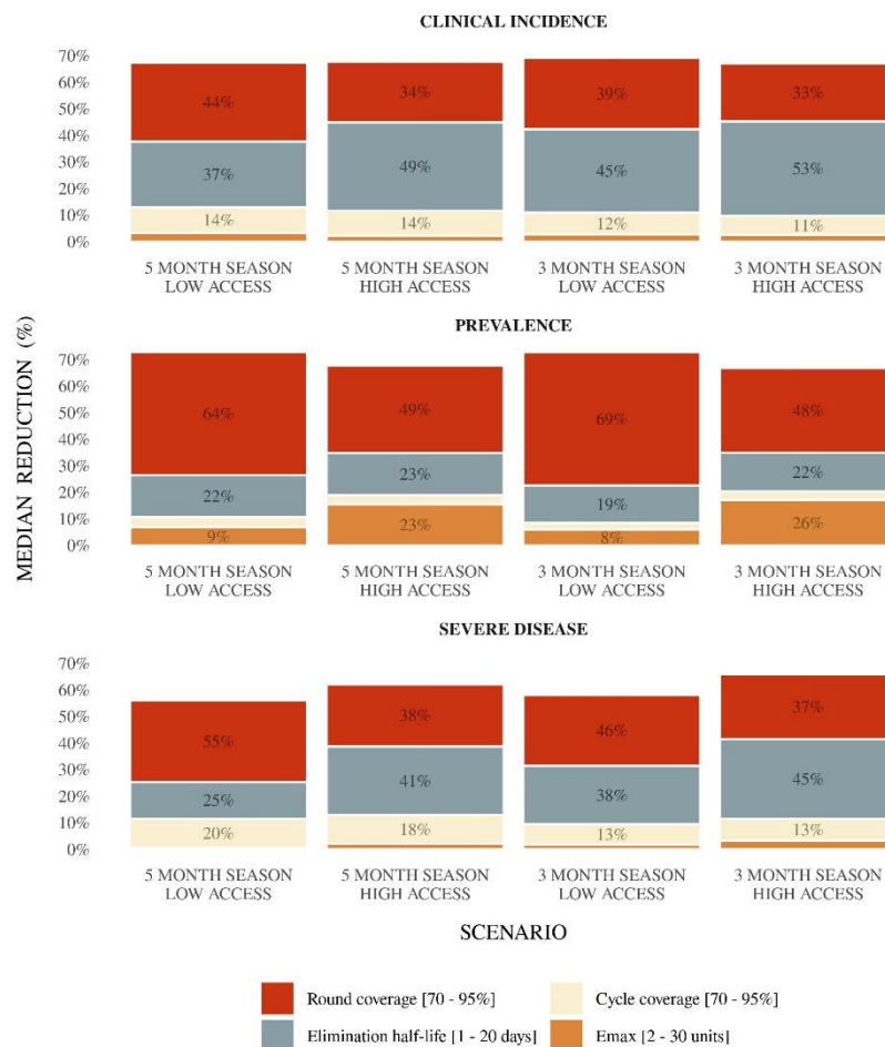
Figure A2.7: For next-generation SMC with dominant blood stage activity and initial, complete liver stage clearance, drivers of impact on predicted levels of reduction of clinical incidence, prevalence, and severe disease for SMC representing four scenarios – low (10%) and high (50%) levels of access to malaria treatment, and three- and five-month seasonal profiles – compared with the no intervention counterfactual. Bars indicate the total Sobol effect indices for key model parameters. Indices can be interpreted as the proportion of variation in the outcome attributable to a given change in each variable, along with its interactions with other variables. Bar heights indicate the median expected reduction across the modelled parameter range. Results are shown for a scenario where SMC is deployed four times at monthly intervals in a given year in children aged three to 59 months, and where the annual baseline PfPR_{2-10} varied with seasonal profile and access from 14% to 24%.
