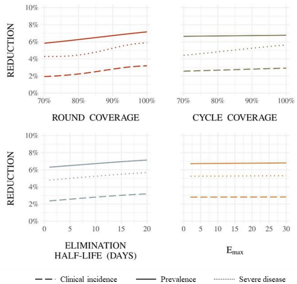
Figure A2.10: For SMC with dominant blood stage activity and initial, complete liver stage clearance, (A) illustrative Gaussian Process regression emulator predictions for the relationship between SMC properties and their direct effects on clinical incidence, prevalence, and severe disease reduction in children aged three to 59 months receiving SMC, and (B) illustrative Gaussian Process regression emulator predictions for the relationship between SMC properties and their indirect effects on clinical incidence, prevalence, and severe disease reduction in children aged 60 to 119 months not receiving SMC
