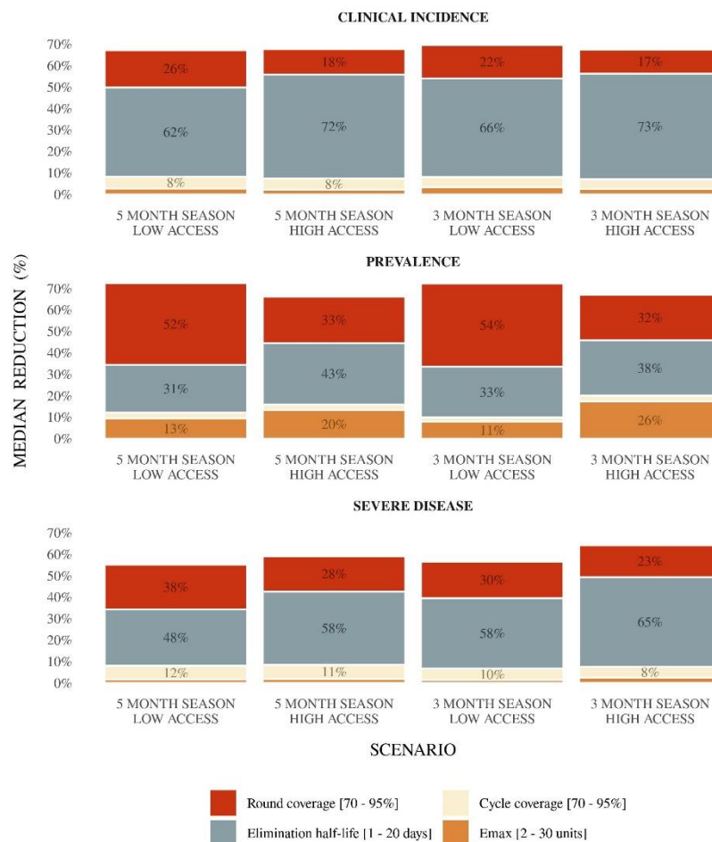
Figure A2.6: For next-generation SMC with blood stage activity only, drivers of impact on predicted levels of reduction of clinical incidence, prevalence, and severe disease for SMC representing four scenarios – low (10%) and high (50%) levels of access to malaria treatment, and three- and five-month seasonal profiles – compared with the no intervention counterfactual
