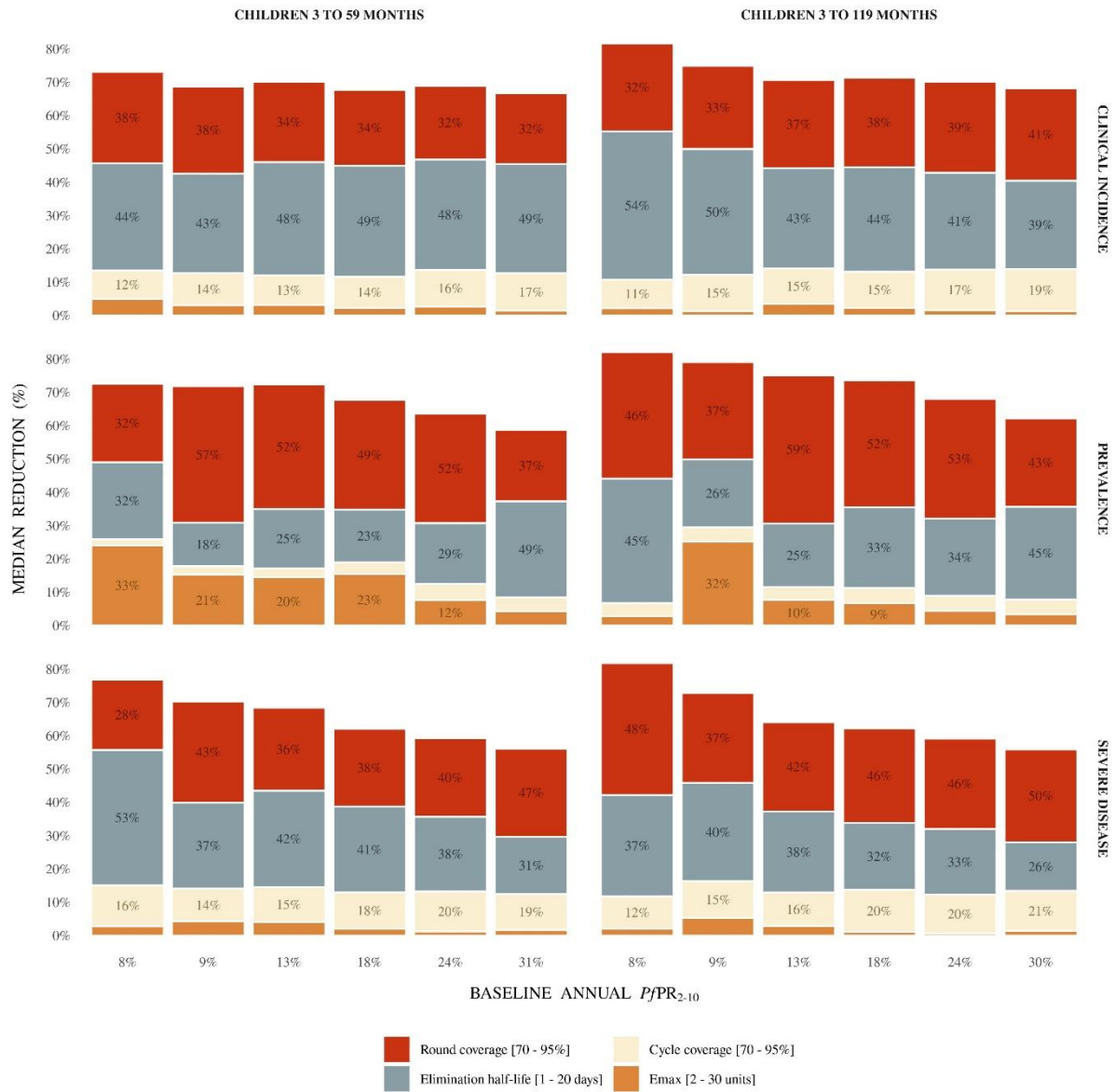
Figure A2.4: For SMC with dominant blood stage activity and initial, complete liver stage clearance, drivers of impact on predicted levels of reduction of clinical incidence, prevalence, and severe disease in two scenarios – delivered to children aged three to 59 months or three to 119 months compared with the no intervention counterfactual
