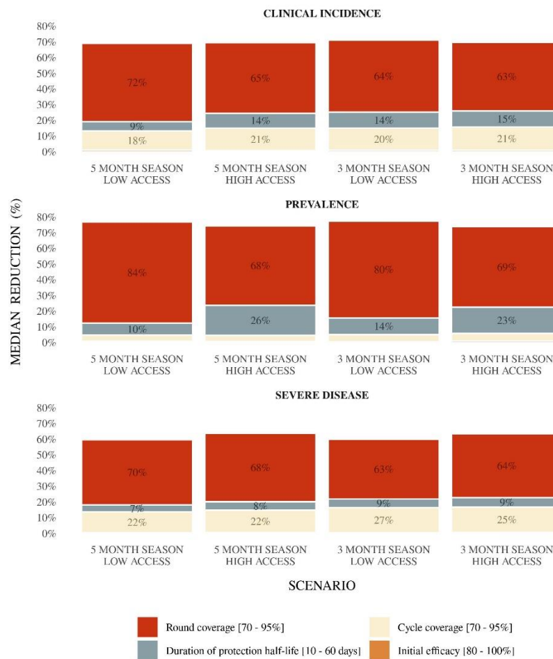
Figure A2.8: For next-generation SMC with dominant liver stage activity and initial, complete blood stage clearance, drivers of impact on predicted levels of reduction of clinical incidence, prevalence, and severe disease for SMC representing four scenarios – low (10%) and high (50%) levels of access to malaria treatment, and three- and five-month seasonal profiles – compared with the no intervention counterfactual. Bars indicate the total Sobol effect indices for key model parameters. Indices can be interpreted as the proportion of variation in the outcome attributable to a given change in each variable, along with its interactions with other variables. Bar heights indicate the median expected reduction across the modelled parameter range. Results are shown for a scenario where SMC is deployed four times at monthly intervals in a given year in children aged three to 59 months, and where the annual baseline PfPR_{2-10} varied with seasonal profile and access from 14% to 24%.
