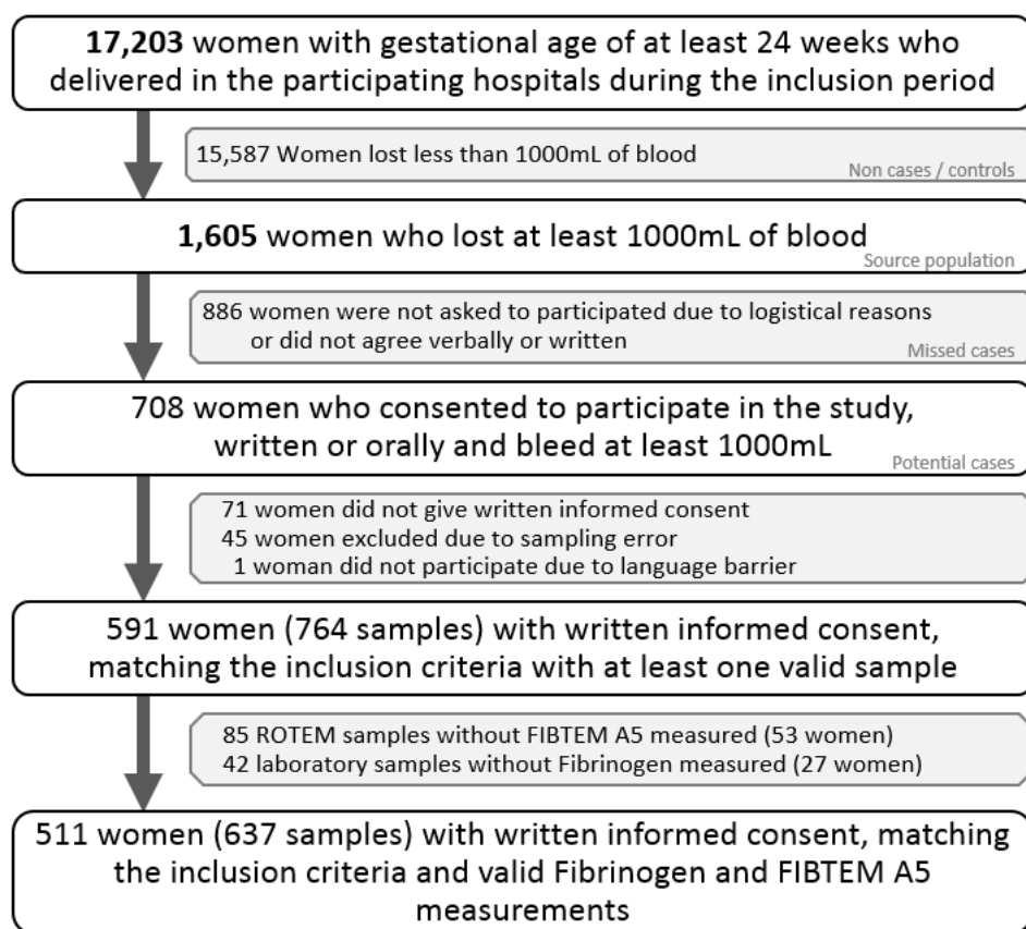
Figure 1: inclusion flowchart
