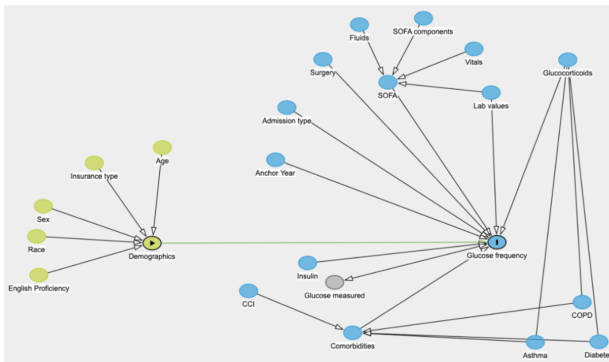
Supplementary Figure 2. Directed acyclic graph for outcome of frequency of glucose measurement over the hospital admission
