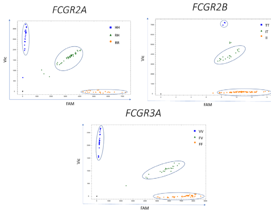
Figure 1. TaqMan
