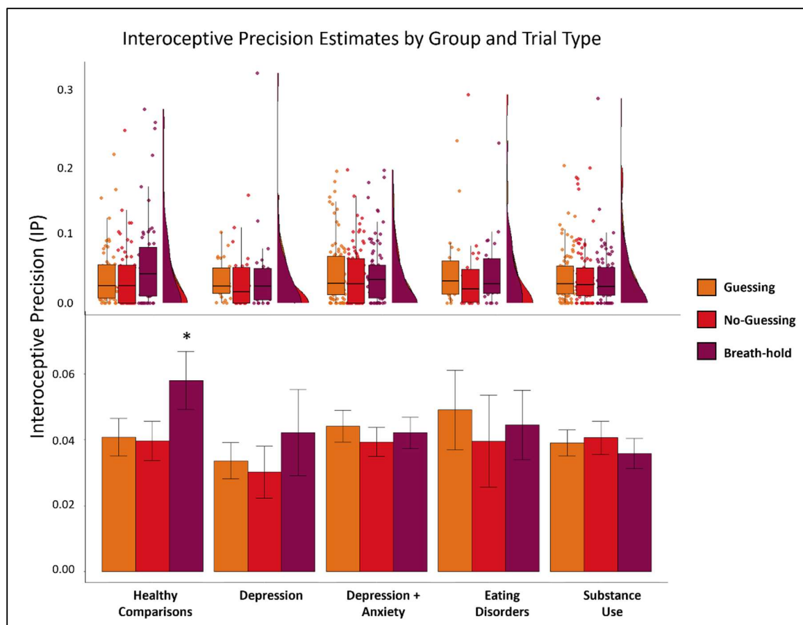
Figure 5. Bottom: Mean and standard error for interoceptive precision estimates by condition and clinical group. The black asterisk indicates that interoceptive precision (IP) was significantly greater in healthy comparisons than other groups (transdiagnostically) in the breath-hold condition, and healthy comparisons showed a significant increase in IP from the guessing and no guessing condition to the breath-hold condition that was absent in the other groups. Top: For more complete data characterization, we also show raincloud plots depicting the same results in terms of individual datapoints, boxplots (median and upper/lower quartiles), and probability densities.
