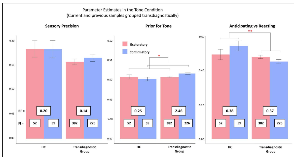
Figure S4. Mean and standard error for model parameters by group and sample in the tone condition. Bayes factors (BFs) comparing samples by group and condition revealed evidence favoring models without a difference between samples in all cases. Linear models (LMs) predicting each parameter in the tone condition with group and sample found a significant effect of sample for pTone ( F(1,715) = 4.52, p = .034 ) such that estimates in the confirmatory sample were higher than the exploratory sample, and a significant effect of group for AvR ( F(1,715) = 6.82, p = .009 ) indicating that healthy controls (HCs) were more reactionary than patients. No significant effects were found for sensory precision ( F_s \leq 3.36, p_s > .067 ).
