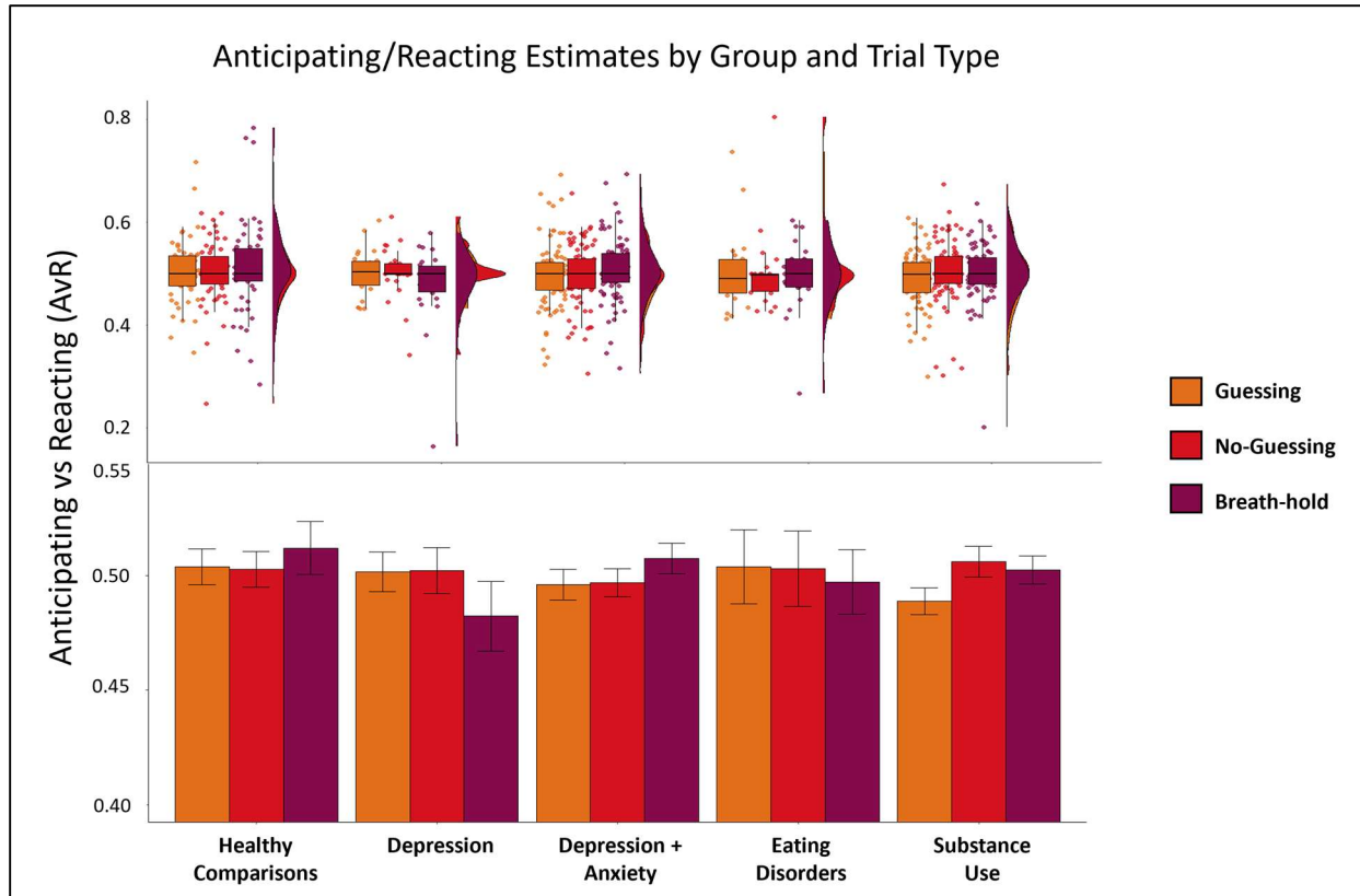
Figure S5. Bottom: Mean and standard error for Anticipating vs Reacting ( AvR ) estimates by condition and clinical group. Top: For more complete data characterization, we also show raincloud plots depicting the same results in terms of individual datapoints, boxplots (median and upper/lower quartiles), and probability densities.
