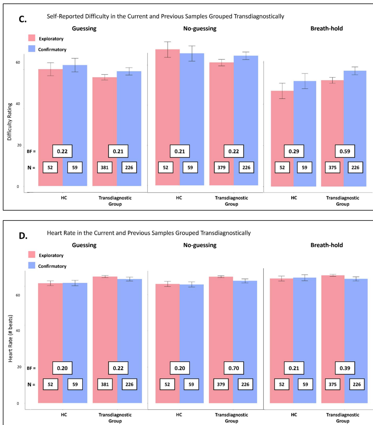
Figure S6. Self-reported task ratings in the confirmatory and exploratory samples across the three heartbeat tapping conditions separated into healthy controls (HCs) and the transdiagnostic patient group. Bayes factors (BFs) comparing samples by group and condition revealed evidence favoring models without a difference between samples in most cases. However, some HC evidence was found suggesting lower confidence ratings in the patient group
