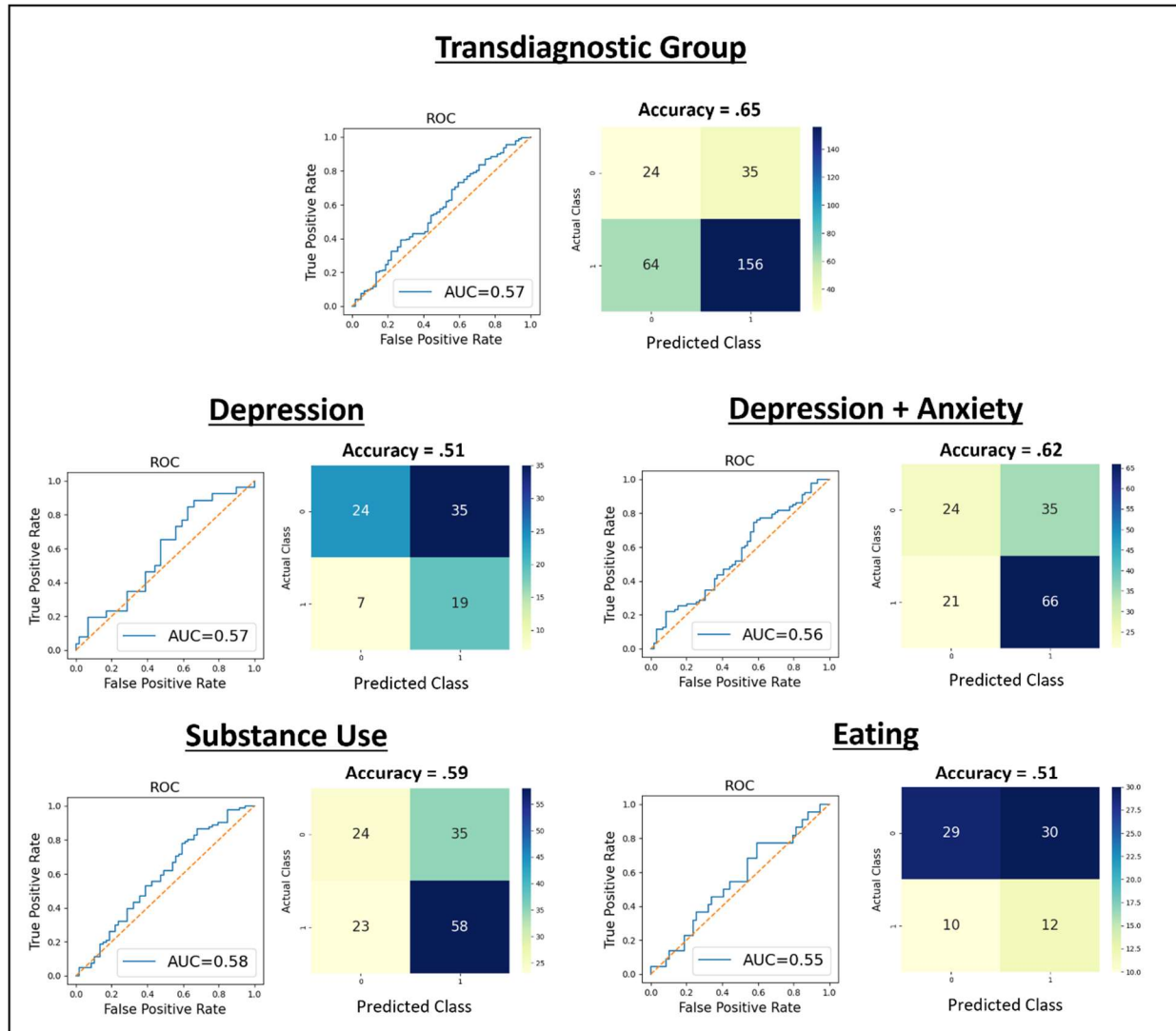
Figure 9. Results of logistic regression models trained on the exploratory sample and then tested on the confirmatory sample (classifying individuals as HCs vs. each patient group). Receiver operating characteristic curves (ROCs) illustrate the true positive rate (sensitivity) vs. false positive rate (1 – specificity) for different categorization thresholds. Performance is quantified by associated area-under-the-curve (AUC) scores, reflecting how often a random sample will be assigned to the correct group with higher probability. Acceptable AUCs vary by application, but the following heuristic cutoff values have been proposed: 0.5 = No discrimination, 0.5-0.7 = Low discrimination, 0.7-0.8 = Acceptable discrimination, 0.8-0.9 = excellent discrimination, > 0.9 = Outstanding discrimination (40). Accuracy at a neutral threshold of 0.5 is also shown in a dotted orange line.
