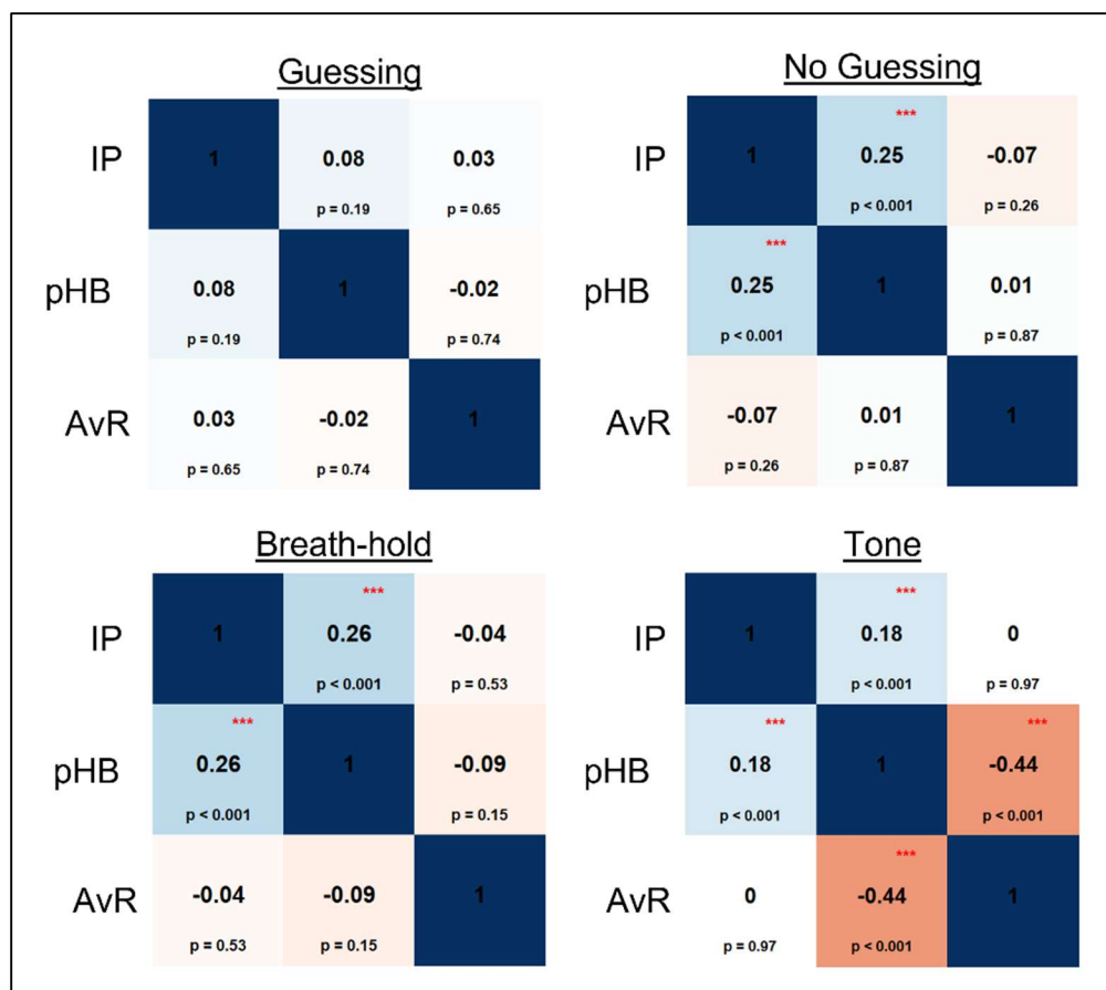
Figure S2. Correlations between model parameters across conditions. IP = interoceptive precision (or sensory precision in the tone condition), pHB = prior expectation over heartbeats (or tone), AvR = anticipating vs reacting.
