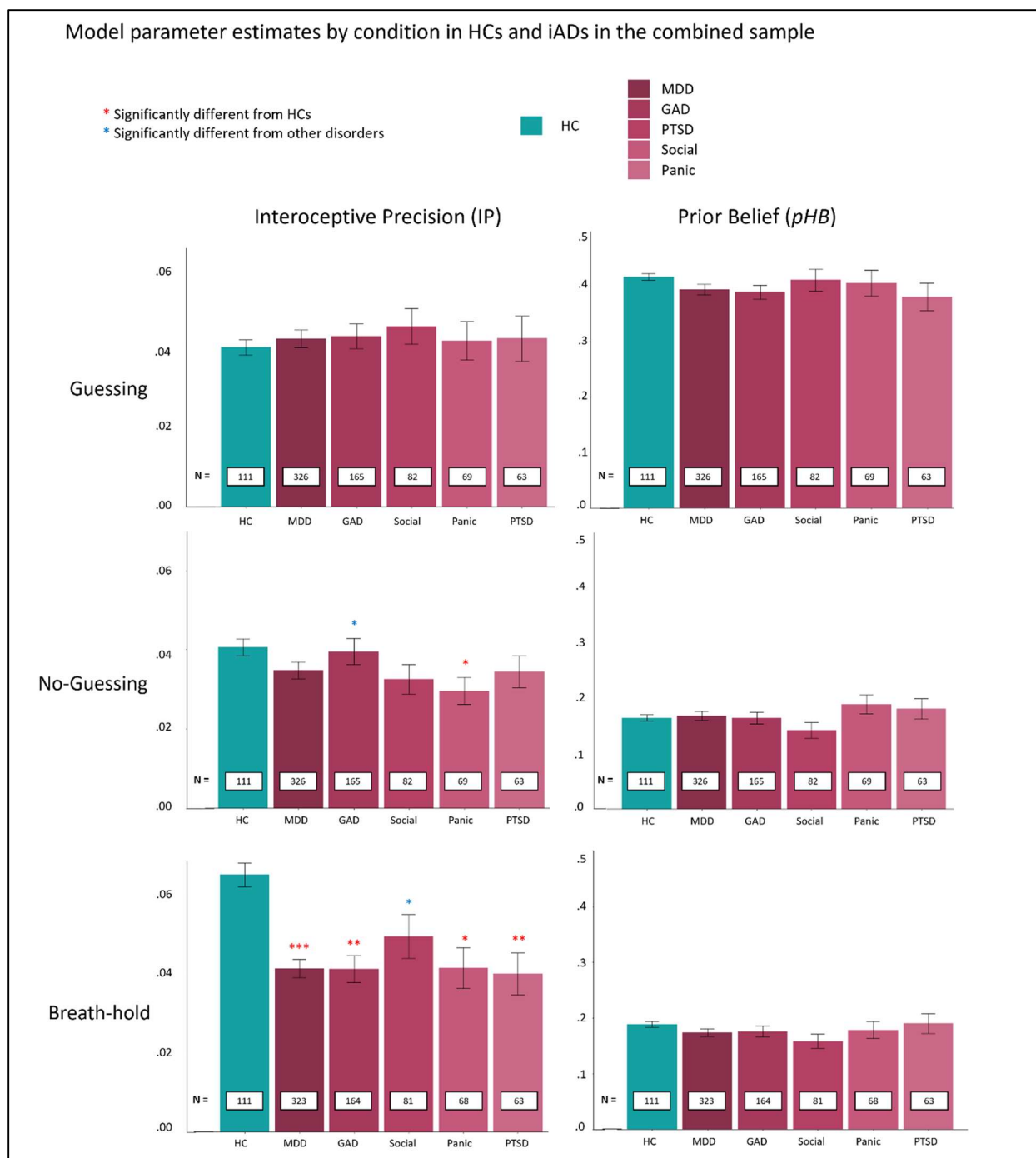
Figure 8. Model parameter estimates ( IP and pHB ) in the three HB tapping conditions in HCs and iADs separated by specific diagnostic groupings.
