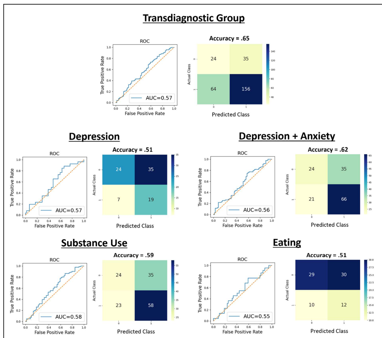
Figure 9. Results of logistic regression models trained on the exploratory sample and then tested on the confirmatory sample (classifying individuals as HCs vs. each patient group). Receiver operating characteristic curves (ROCs) illustrate the true positive rate (sensitivity) vs. false positive rate (1 – specificity) for different categorization thresholds. Performance is quantified by associated area-under-the-curve (AUC) scores, reflecting how often a random sample will be assigned to the correct group with higher probability. Acceptable AUCs vary by application, but the following heuristic cutoff values have been proposed: 0.5 = No discrimination, 0.5-0.7 = Low discrimination, 0.7-0.8 = Acceptable discrimination, 0.8-0.9 = excellent discrimination, > 0.9 = Outstanding discrimination (40). Accuracy at a neutral threshold of 0.5 is also shown in a dotted orange line.
