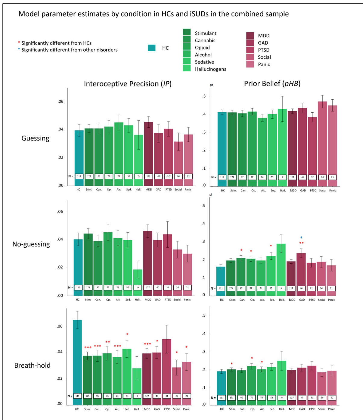
Figure 7. Model parameter estimates ( IP and pHB ) in the combined exploratory/confirmatory dataset in the three HB tapping conditions in HCs and iSUDs, separated by specific diagnostic groupings. Note that these groupings contain overlapping participants as they include anyone with a given diagnosis irrespective of co-morbid diagnoses. Red asterisks indicate groups differentiable from HCs in logistic regressions. Blue asterisks indicate diagnostic groups that could be differentiated from other diagnoses in similar logistic regressions (excluding HCs). Detailed results of these analyses can be found in Supplementary Tables S2 and S3 .
