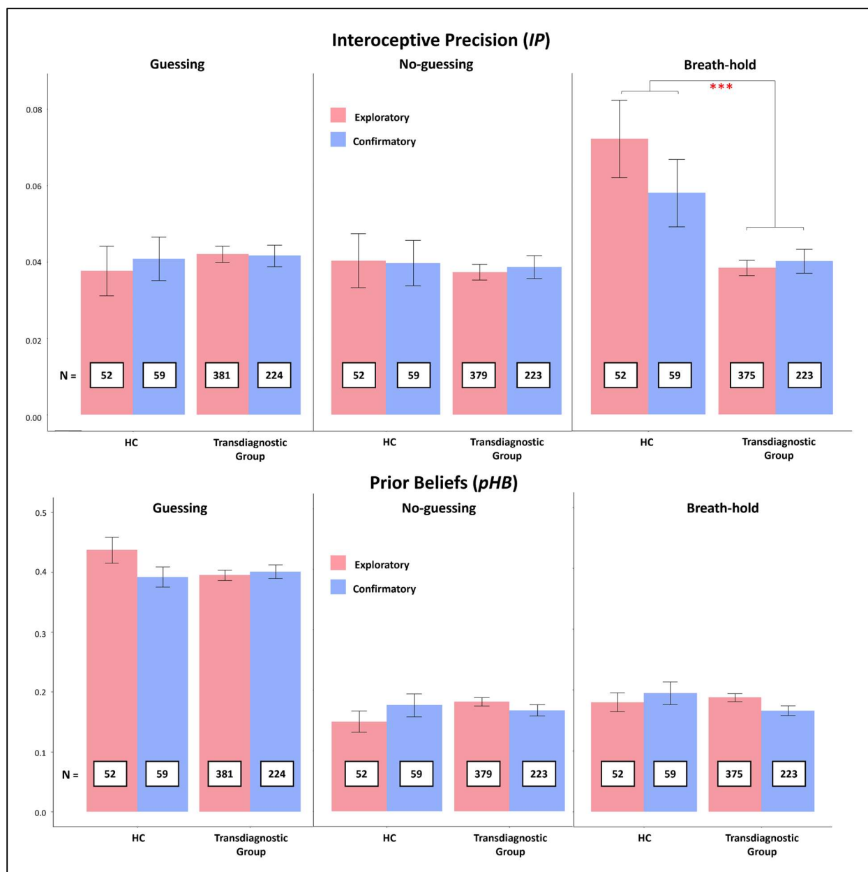
Figure 4. Top: Interoceptive precision (IP) estimate comparison between the previous (i.e., exploratory) and current (i.e., confirmatory) samples when grouping participants transdiagnostically. Red asterisks indicate a significant difference ( ***p < .001 ) in IP estimates within an LME between groups in the breath-hold condition (but no difference between samples in either group). Bayes factor analyses also provided moderate to strong evidence supporting an absence of differences between samples in all cases: BFs between .09 (Guessing Condition, Patients) and .33 (Breath-hold Condition, HCs). Bottom: Prior expectation (pHB) estimate comparison between the previous (i.e., exploratory) and current (i.e., confirmatory) samples when grouping participants transdiagnostically. No significant differences between groups or samples were observed. Bayes factor analyses also provided evidence supporting an absence of differences between samples in all cases: BFs between .10 (Guessing Condition, Patients) and .69 (Guessing Condition, HCs; Breath-hold Condition, Patients).
