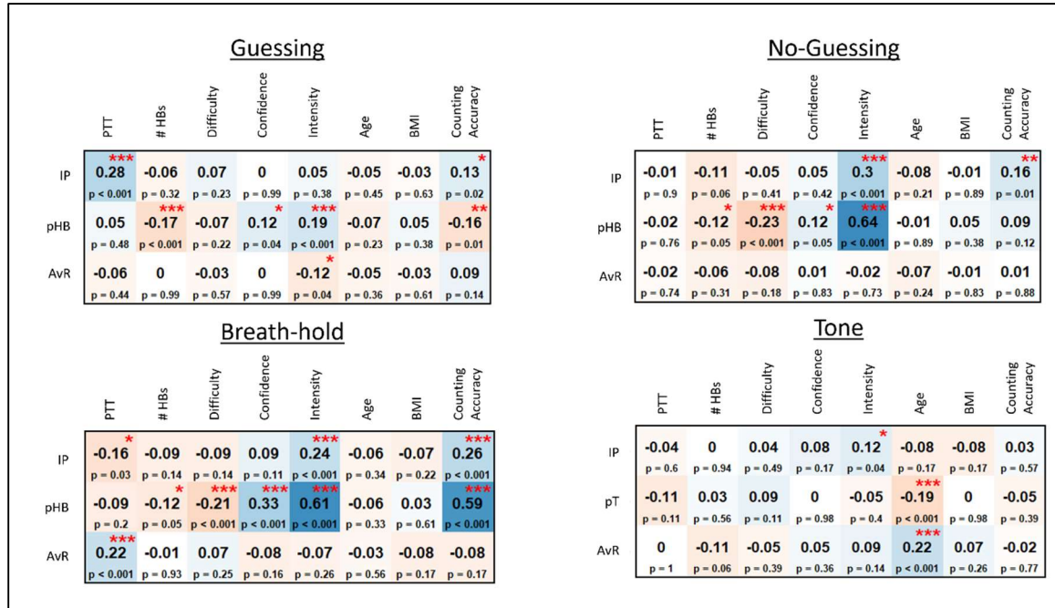
Figure 3. Exploratory Pearson correlations between model parameters and self-report and other task-relevant variables for each task condition across all participants. IP = interoceptive precision parameter, pHB = prior belief for heartbeat parameter, pT = prior belief for tone parameter, AvR = anticipate vs. react strategy parameter, PTT = median pulse transit time, #HBs = number of heartbeats during the task condition, BMI = body mass index. For reference, significant correlations are marked with red asterisks: * p < .05 , ** p < .01 , *** p < .001 .
