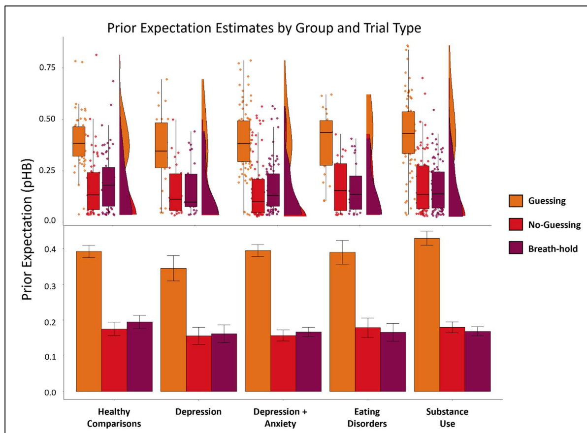
Figure 6. Bottom: Mean and standard error for pHB estimates by condition and clinical group. Top: For more complete data characterization, we also show raincloud plots depicting the same results in terms of individual datapoints, boxplots (median and upper/lower quartiles), and probability densities.
