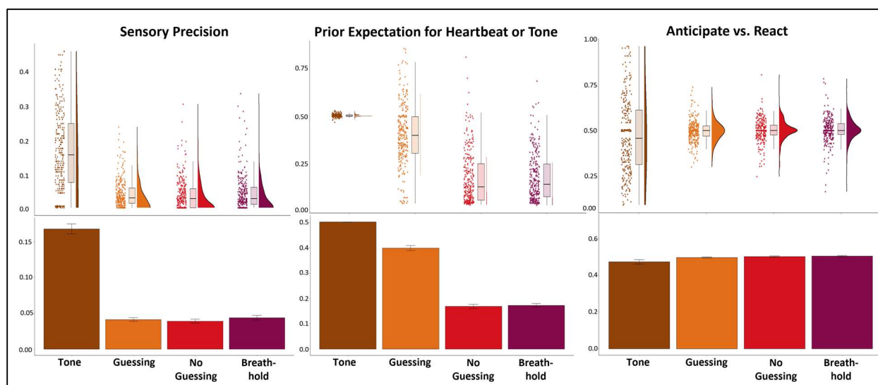
Figure S1. Bottom: Bar plots comparing means and standard errors for model parameters in the tone condition to those in the HB conditions. Prior beliefs for tones reflected no bias. Sensory precision for the tone condition was high, which was expected given the unambiguous nature of this signal relative. The Anticipate vs. React parameter in the tone condition did not significantly differ from the HB conditions, but had greater variance. Top: For more complete data characterization, we also show raincloud plots depicting the same results in terms of individual datapoints, boxplots (median and upper/lower quartiles), and distributions. These further illustrate that, for the Anticipate vs. React parameter, nearly equally sized clusters of participants appeared to adopt more anticipatory (<.5) vs. reactive (>.5) strategies in the tone condition, and that prior beliefs remained unbiased (.5; with little variance) in the tone condition relative to the HB conditions. This pattern of results matched that found in our previous study.
