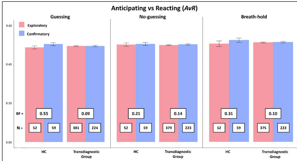
Figure S3. Mean and standard error for Anticipating vs Reacting ( AvR ) in the three heartbeat tapping conditions. Bayes factors (BFs) comparing samples by group and condition revealed evidence favoring models without a difference between samples in all cases. Linear models (LMs) predicting AvR in each condition with group and sample found no significant effects or interactions ( F \leq 1.95 , p \geq .163 in all cases).
