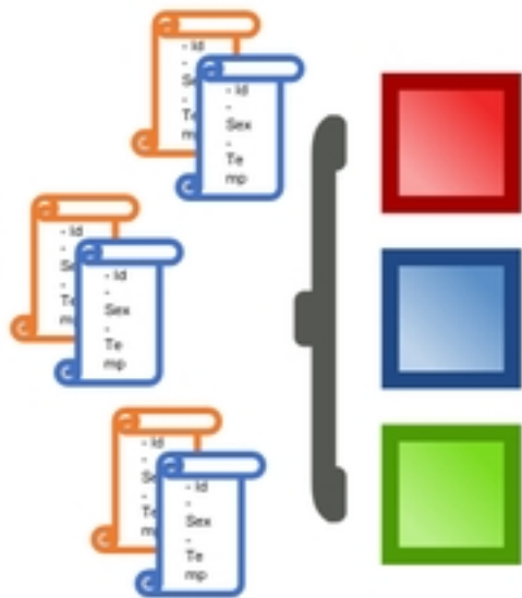
Figure 1. Harmonization Process
