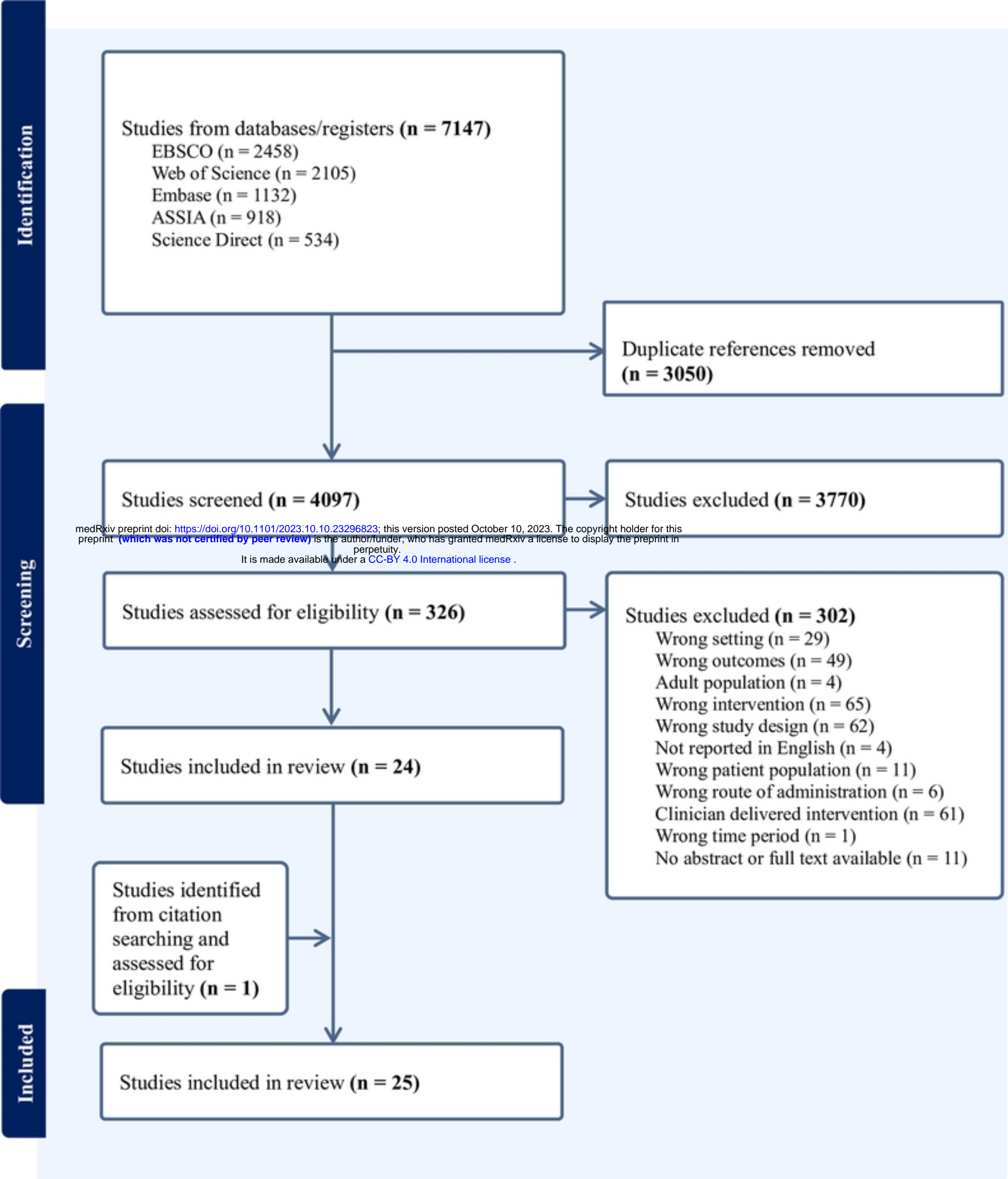
Fig 1. PRISMA diagram
