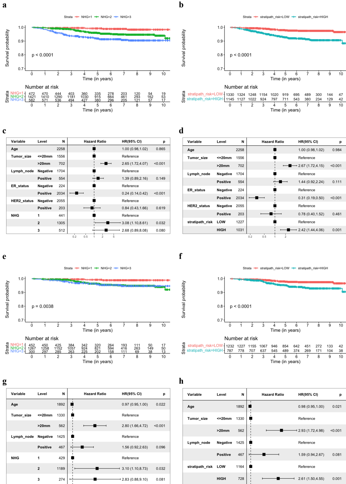
Figure 2. Prognostic stratification of patients by clinical NHG and Stratipath Breast. a Kaplan Meier (KM) curves for progression-free survival (PFS) among all patients stratified
