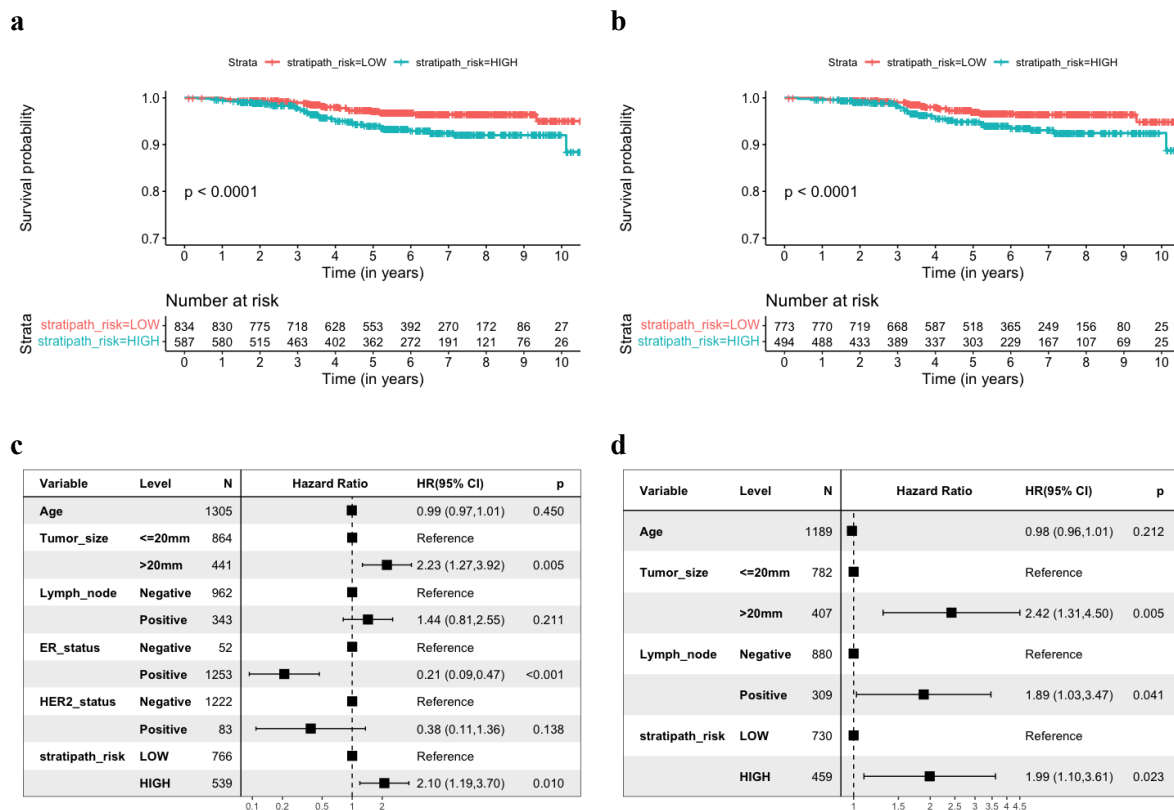
Figure 3. Prognostic stratification of patients with intermediate grade (NHG2) using
