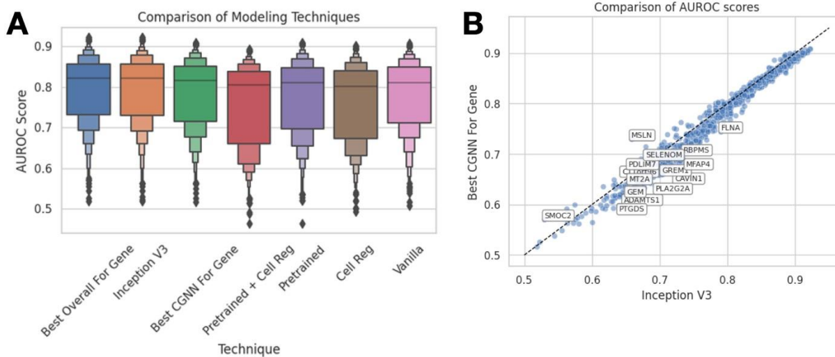
252 Figure 3: Performance comparison between methods. A) Boxplot of AUROC scores from each 253 method; B) comparison of AUROC for best CGNN and CNN for each gene
