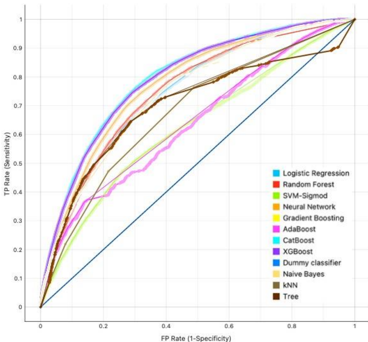
Figure 2. AUROC curve analysis of machine learning algorithms for prediction of MACE in family medicine patients.
