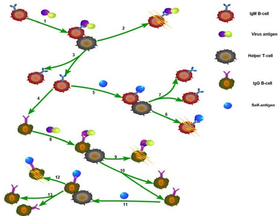
Figure 1 : Model schematic. 13 core reactions and 5 components are illustrated in the model. Those 5 components include virus antigen, self-antigen, IgM-producing B-cell, IgG-producing B-cell, and helper T-cell. Each reaction is represented in green line with arrow indicating the reaction direction.
