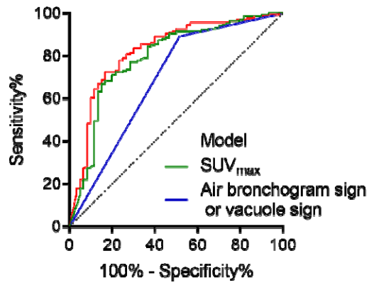
Fig. 3 ROC curve of the model built on SUV max and air bronchogram sign or vacuole sign for preoperative predicting IASLC grade 3 tumor.
