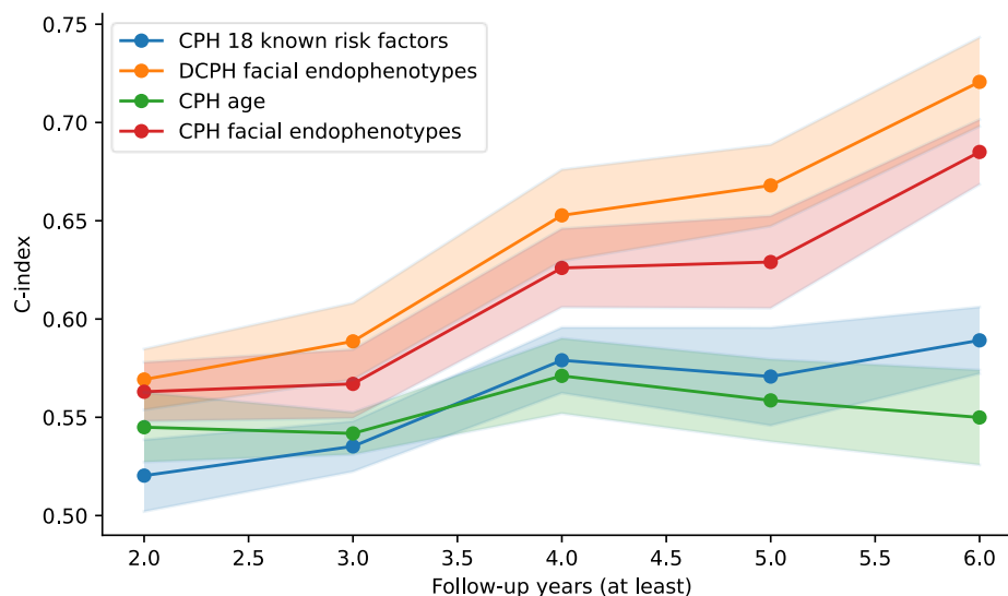
397 398 Figure 4: Stratification of right-censored samples based on follow-up years. The solid line represents the mean 399 result, while the transparent surrounding area denotes the standard deviation. (CPH 18 known risk factors): Results 400 obtained from a CPH model using risk factors as predictors. (DCPH facial endophenotypes): Results obtained from a 401 DCPH model using facial endophenotypes as predictors. 402
