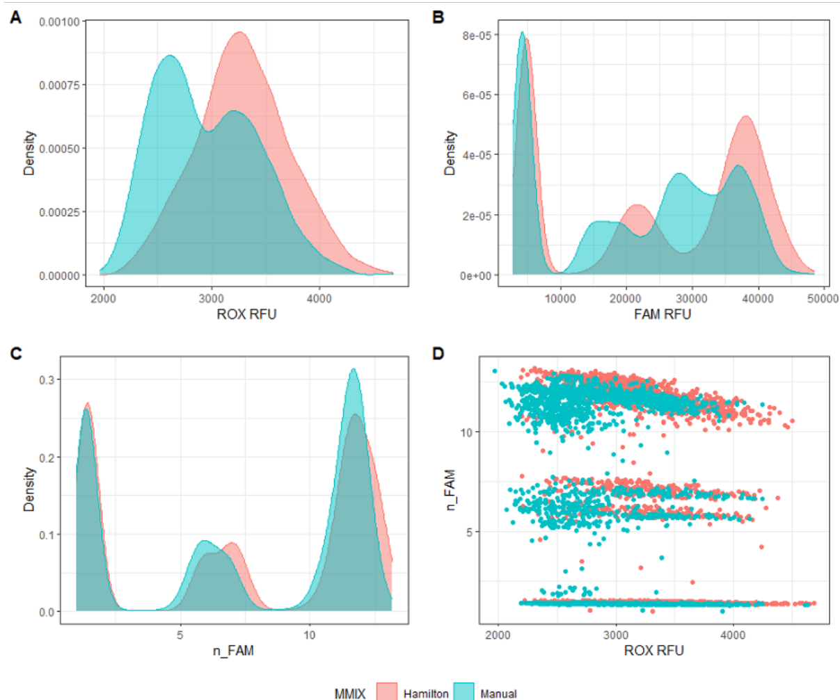
Figure 10: StarLet-Prepared MMIX compared with Manually-Prepared MMIX. End-point RFU data from PCR reactions using dilutions of synthetic RNA positive control material (Seracare AccuPlex) at and around the limit of detection. A) ROX RFU kernel distribution B) FAM RFU kernel distribution. C) n_FAM kernel distribution. D) Scatterplot n_FAM vs ROX RFU. Data are pooled from six 384-well arrays for both conditions.
