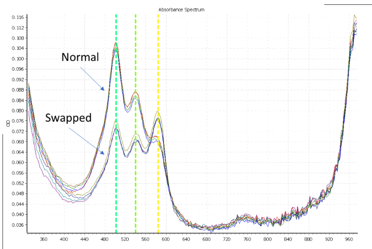
Figure 4: ABS scan, comparing the absorption spectra of “Normal” MMIX, and a “Swapped” MMIX, where the volumes of the ROX and OLIGO are exchanged. N = 4.
