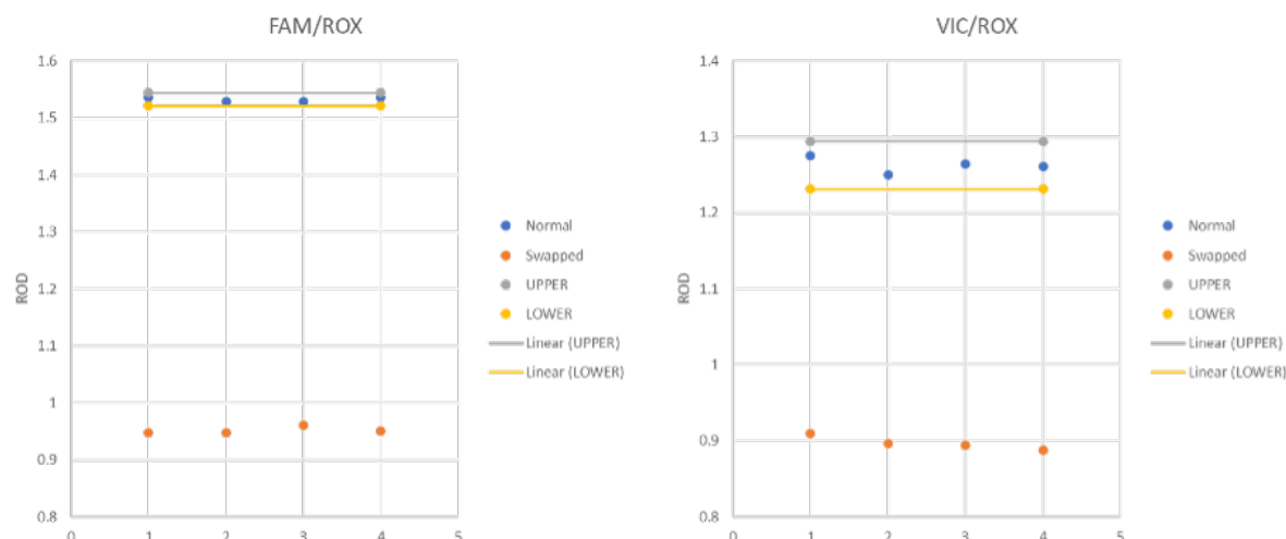
Figure 5: Ratio of FAM/ROX and VIC/ROX, with upper and lower limits defined as \pm 3 SD from the mean. N = 4.
