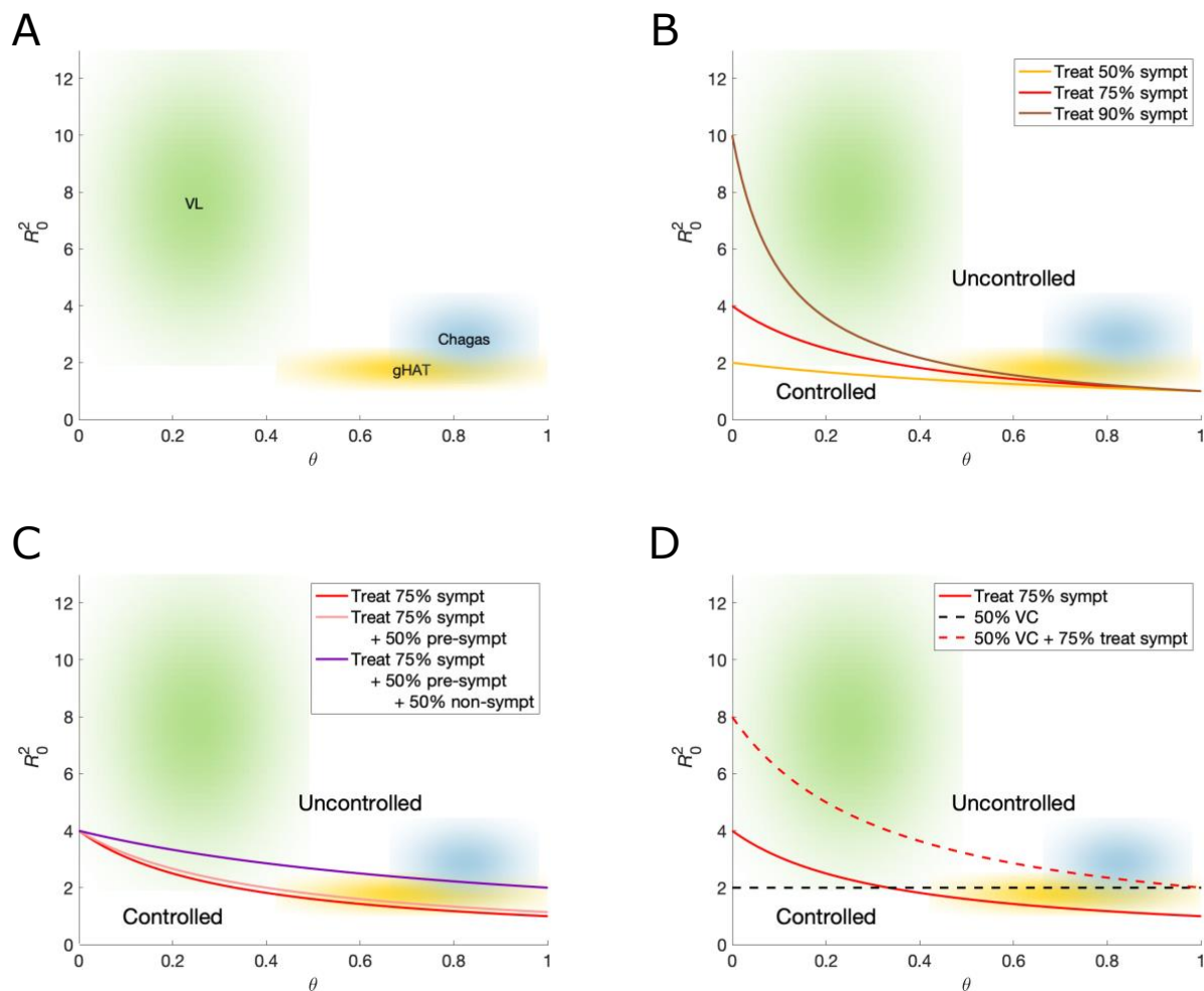
Figure 2. Potential for control of VL, gHAT and Chagas disease under different combinations of generic interventions. (A) Plot illustrating the relative position of each of VL (green), gHAT (yellow), and Chagas disease (blue) in the phase space determined by the full-cycle reproduction number of the disease, R_0^2 (the average number of secondary infections caused by one infectious individual in an entirely susceptible population), and the proportional contribution of non-symptomatic and pre-symptomatic individuals to R_0^2 , \theta . Clouds represent parameter uncertainty. (B)–(D) Sensitivity of the diseases to different interventions. The curves delineate successful control (below the line) with each intervention: (B) treating symptomatic individuals; (C) treating symptomatic individuals and pre-symptomatic and/or non-symptomatic individuals; (D) vector control (VC) – achieving 50% vector control corresponding to halving the vector population, reducing the bite rate or shortening vector life expectancy.
