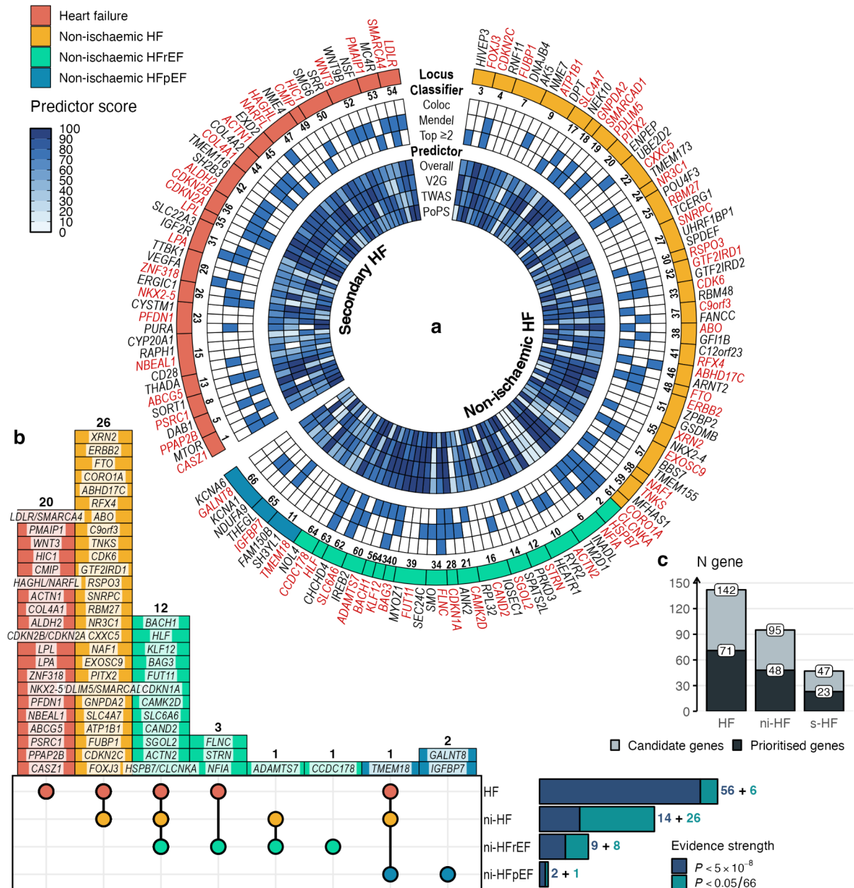
Figure 2. a. Sunburst chart of Candidate genes (black label) and Prioritized genes (red label) for HF identified through gene prioritisation strategy across 66 loci showing heatmap of predictor score and boolean classifier score (blue tile indicates a ‘True’ value). b. Upset plot showing number of loci categorised by phenotypic associations across HF subtypes, colour coded by the most specific association at P < 0.05 / 66 and labelled with Prioritized genes. c. Number of Candidate and Prioritized genes across HF phenotype gene set.
