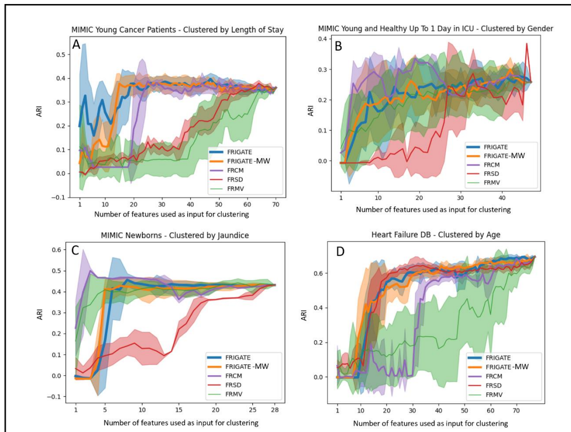
Figure 4. A-D: Performance on datasets 5-8 respectively. See Figure 3 for caption details.
