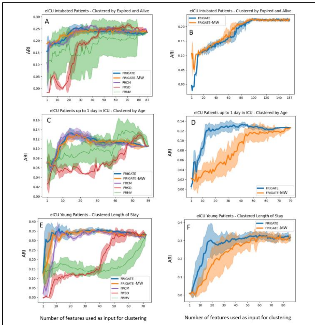
Figure 5. Performance on datasets 9-12 from the eICU repository. See Figure 3 captions for details. A-B: dataset 9, C-D: dataset 10, E-F: dataset 11. A, C, E show results when using only the continuous features of the datasets, and B, D, F show results for the mixed data.
