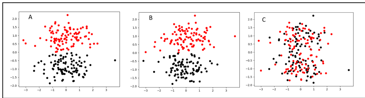
Figure 2. Illustrations of the different steps of FRIGATE for scenario 2 that is shown in Figure 1B, where one feature is informative (y axis) and one is non-informative (x axis). A – a clustering solution of the data (line 6 in Algorithm 1) colored by clusters labels. The solution score is 237.28 (line 8 in Algorithm 1). B- Results of shuffling the x coordinates, representing the non-informative feature (lines 10-13 in Algorithm 1). The solution score is similar to A and the feature’s score is 0.51. C- Results of shuffling the y coordinates, representing the informative feature. An increase in the solution score led to a feature’s score of 304.5.
