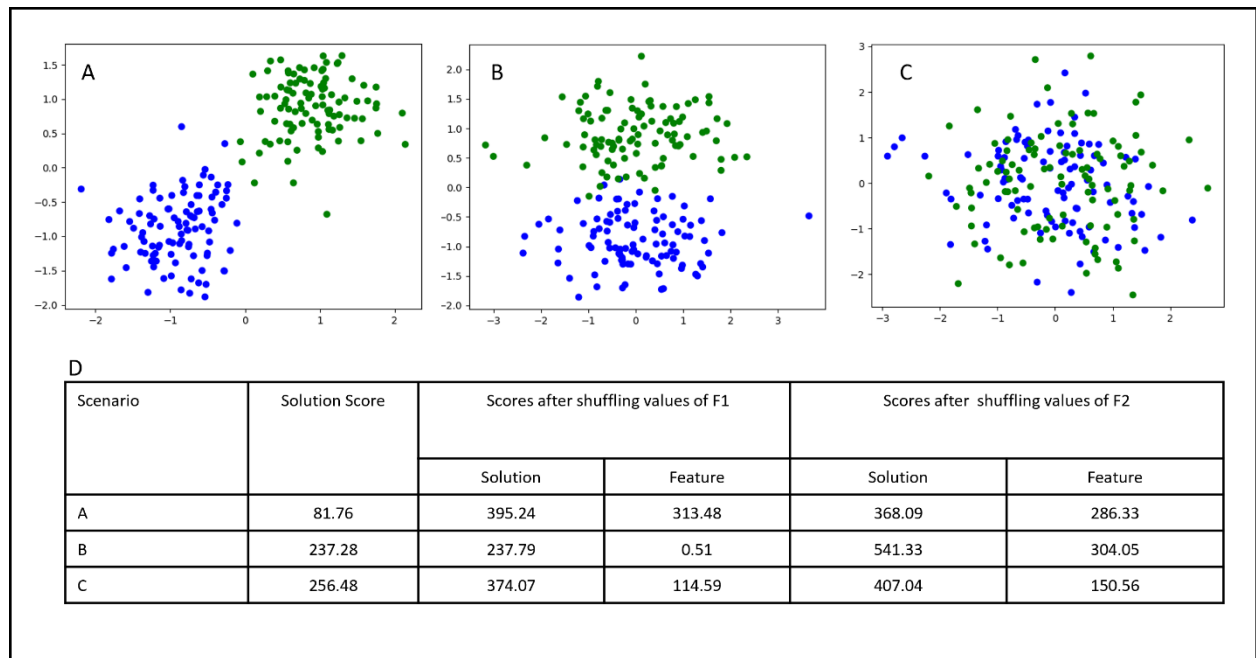
Figure 1. Illustrations of simulations with two clusters. In the simulation, there are 100 samples in each cluster, \mu = 4 , \sigma = 0 , and two features. A-C: features are represented by the axes. Each color represents a different cluster. A: both features are informative for clustering, B: only the feature represented by the y axis is informative, C: both features are not informative. D: Demonstration of FRIGATE iteration on the data of A-C. Solution score refers to line 8 in Algorithm 1, feature's score refers to line 13 in Algorithm 1. F1 is represented by the x-axis in Figure1 A-C and F2 is represented by the y-axis. We can see that the informative features received higher scores than the non-informative ones.
