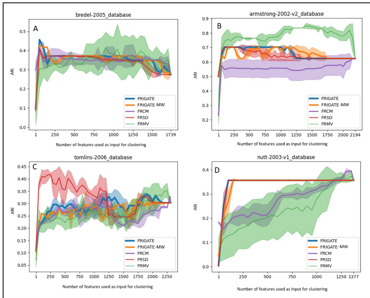
Figure 3. Performance of the tested algorithms on genomic datasets. The ranking produced by each algorithm was used to cluster the data with a growing number of features. The Y axis is the ARI score compared to the known clustering. The results are average of ten runs. The light-colored sleeve around each plot is \pm 1 std. A-D for datasets 1-4 in Table 2, respectively.
