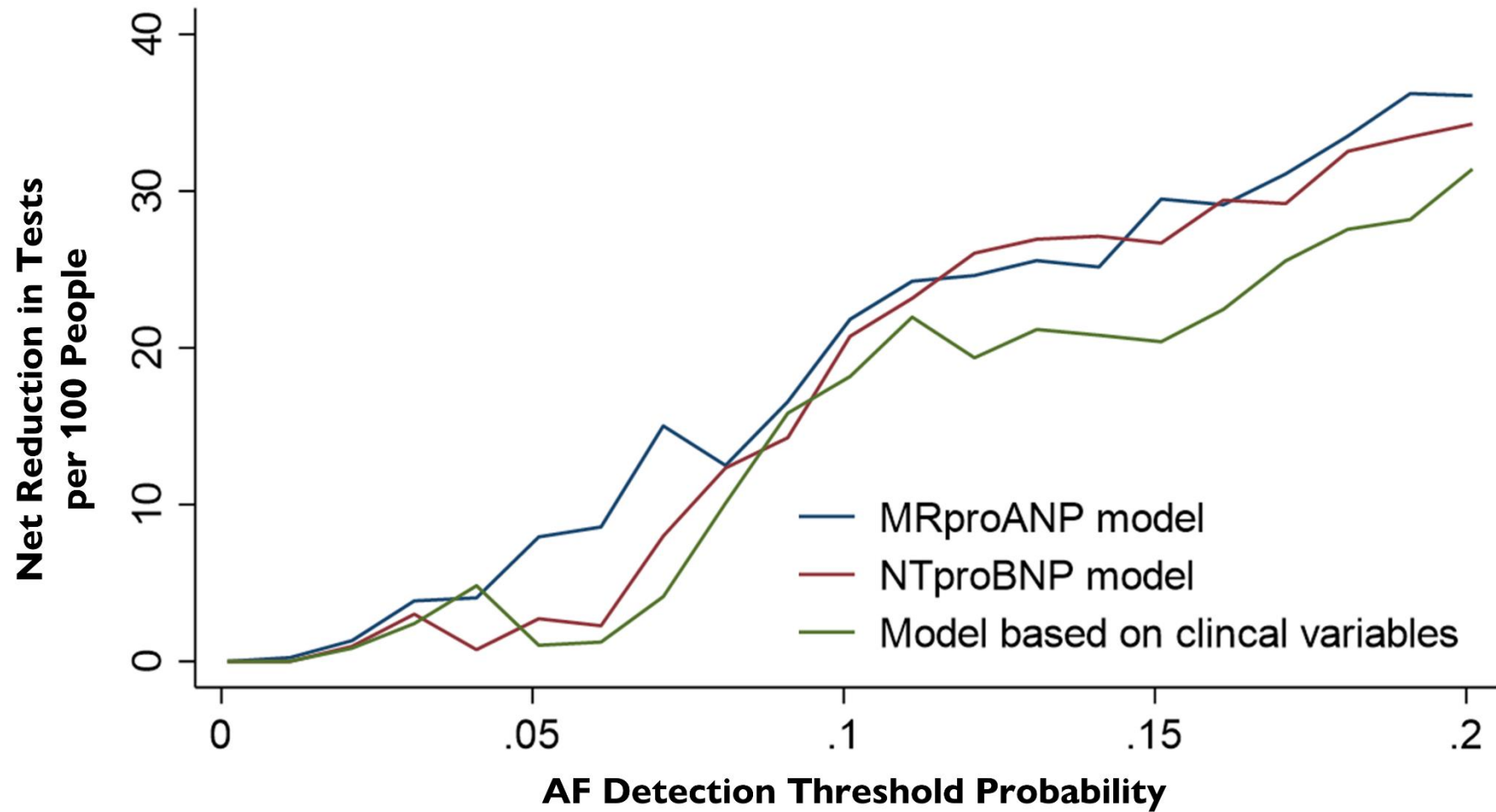
Figure 1. Decision Curve Analysis for Net Reduction in the Number of People who Would Need Prolonged Cardiac Monitoring
