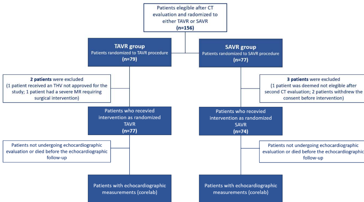
Figure 1. Study flowchart
