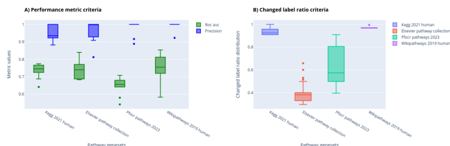
Fig. 5 Evaluation of all types of pathway gene sets (pfocr, kegg, elsevier, wikipathways) according to the roc auc and precision metrics for the model quality criteria, and following the changed label ratio on calibrating by clinical trial drugs.
