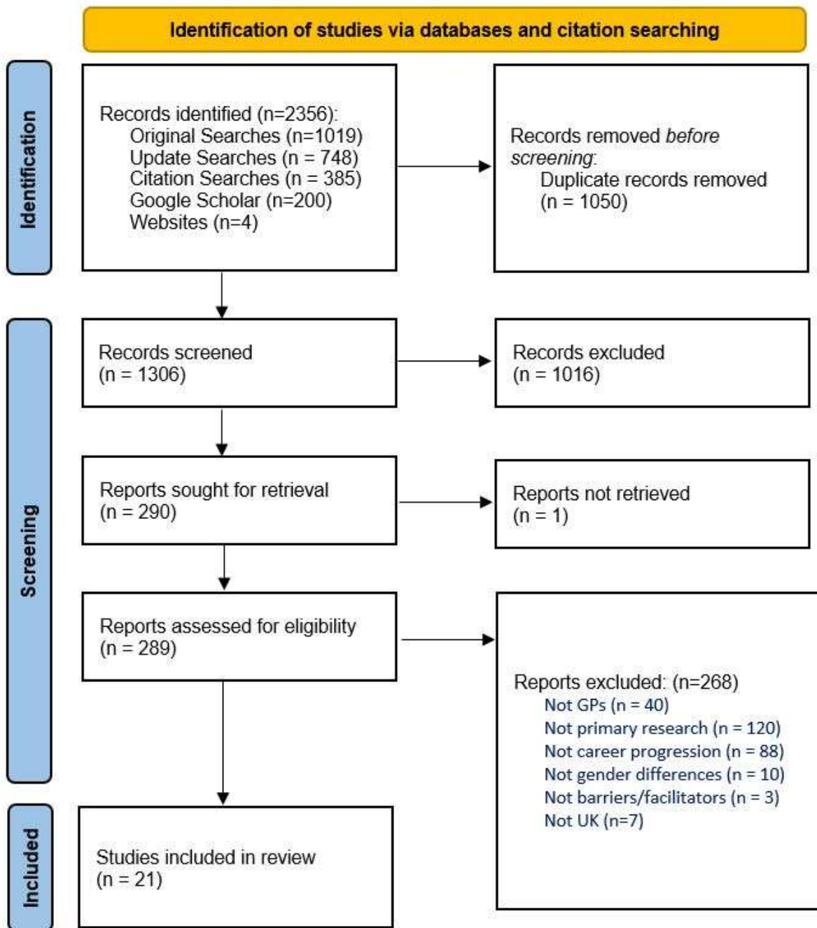
Figure 1: PRISMA diagram
