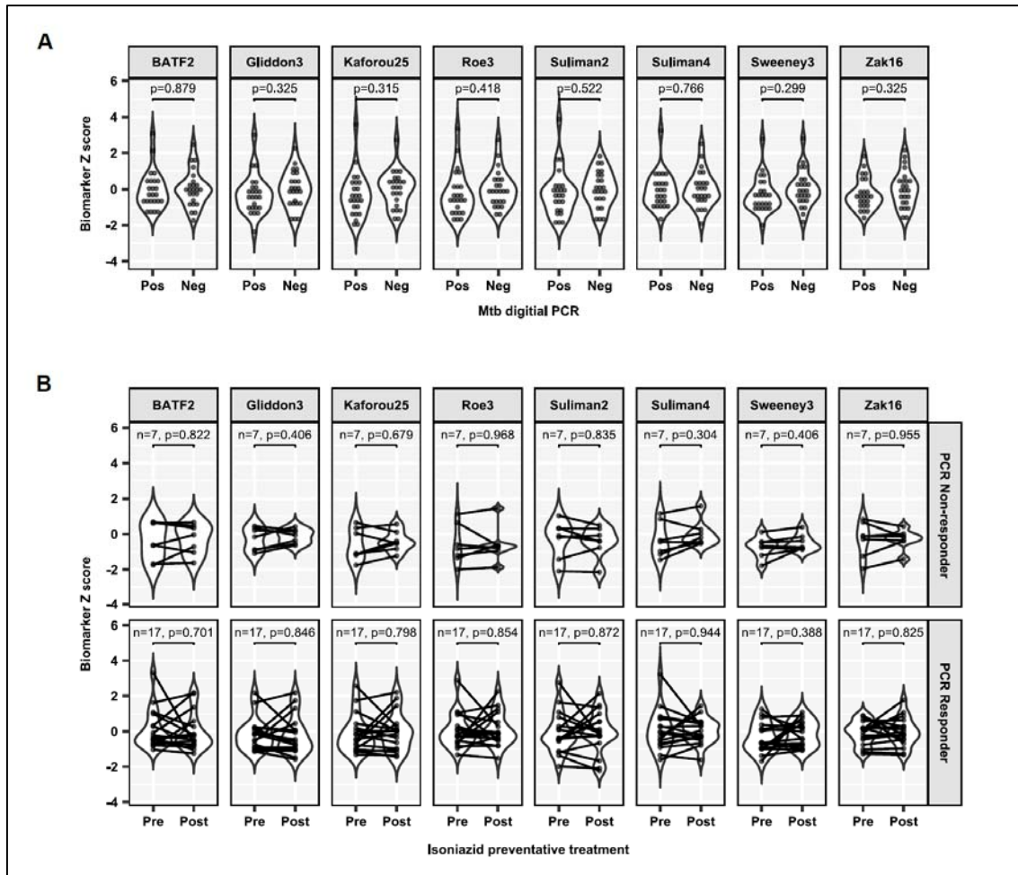
Figure 1: Z-scores for expression of eight different signatures for incipient TB in whole blood of asymptomatic adults in Ethiopia. A, Baseline Z-scores by Mtb DNA status. B, Z-scores before vs. after administration of isoniazid preventive therapy among those in whom Mtb DNA was detected at follow-up ('PCR non-responders', top row) and those in whom Mtb DNA was undetectable at follow-up ('PCR responders', bottom row).
