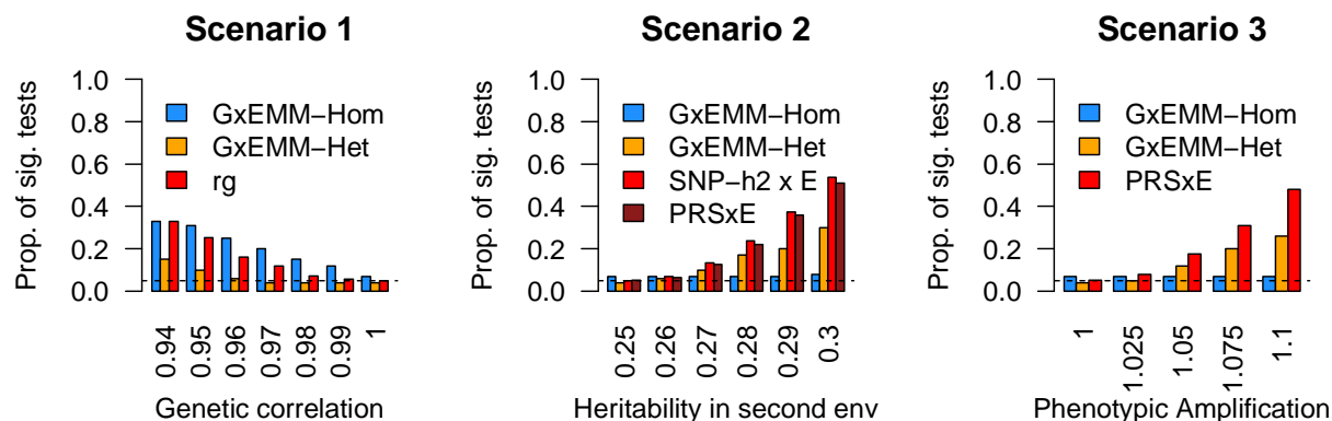
919 Figure S2 Comparison of three statistical approaches for detecting GxE to ExEMM in 920 simulations. a) Scenario 1 with varying true genetic correlation across E, b) Scenario 2 with 921 varying heritability in the second environment, c) Scenario 3 with phenotypic amplification 922 across E bins. 923 924
