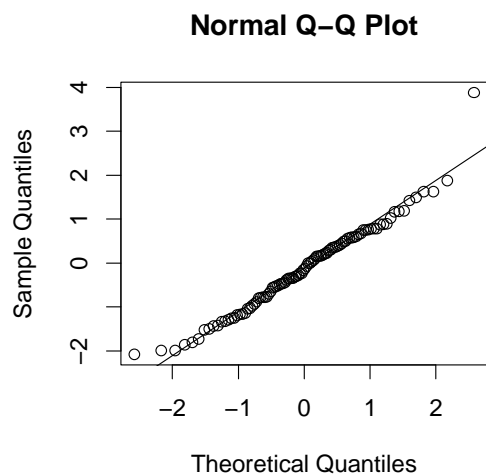
925 926 Figure S3 Null simulations of a heritable and genetically correlated E variable. We 927 simulated an E variable that is 100% genetically correlated to the phenotype with the same 928 heritability ( h^2=25\% ). Each point is the result of a PRSxE regression test from a single 929 simulation (N=100 simulations). We find no inflation of the test statistic under this null model. 930
