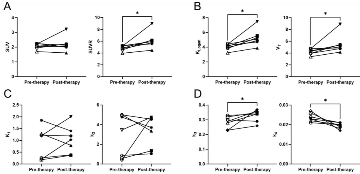
FIGURE 7. Changes in seven sub-regions of the LLL tumor post-therapy, using (A) SUVmean or SUVR values without kinetic modeling, (B) K_{Logan} from Logan plots or V_T from 2T6P compartmental modeling as macroparameters with high identifiability, (C) 2T6P rate constants between blood and first compartment ( K_1 and k_2 ), and (D) 2T6P rate constants between first and second compartments ( k_3 and k_4 ).
