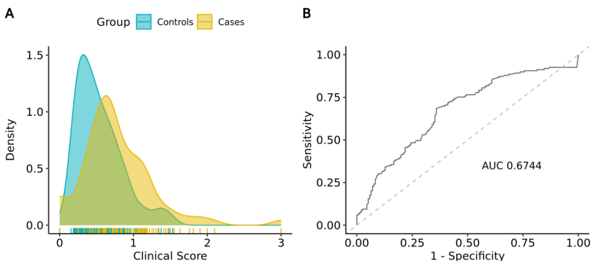
Figure 3: Distribution curve and predictive accuracy of the 5-year clinical risk score. (A) Distribution curve of the clinical risk score in cases vs. controls. Higher scores ( 0.76 \pm 0.44 ) are observed in cases compared to controls ( 0.54 \pm 0.31 ), with the difference being statistically significant (p-value: 5.16 \times 10^{-4} ). (B) ROC curve for the clinical risk score. The observed AUC is 0.674.
