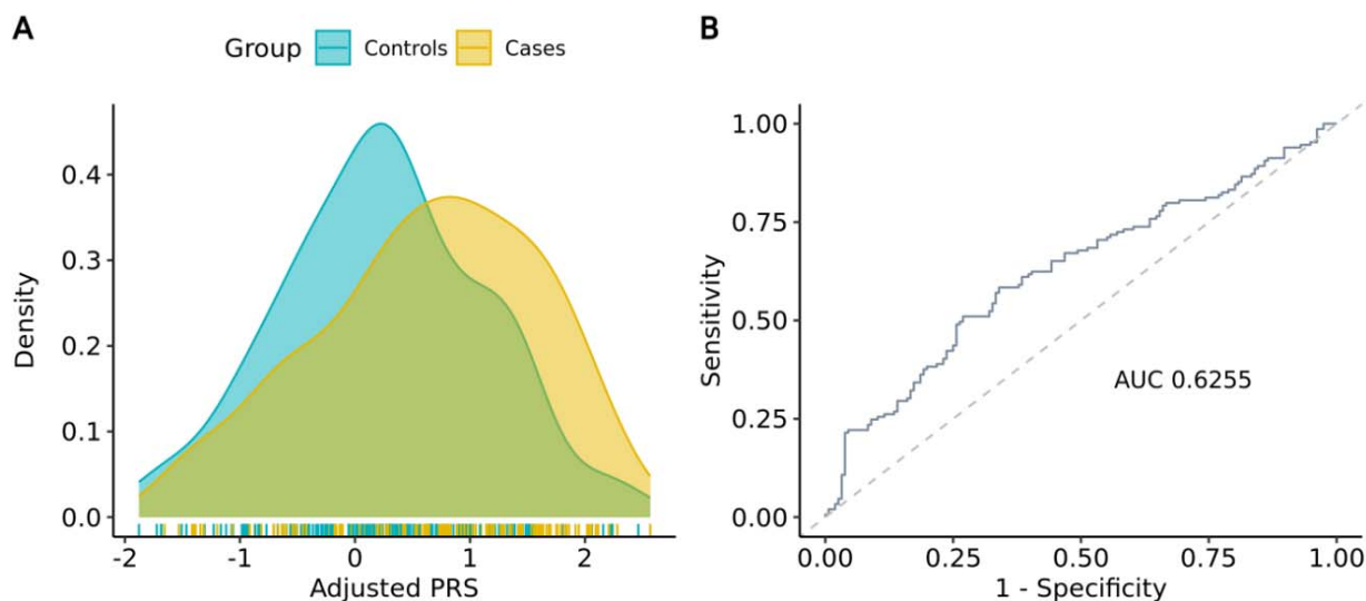
Supplementary Figure 2: Distribution curve and predictive accuracy of ancestry-adjusted PRS. (A) Distribution curve of adjusted PRS in cases vs. controls. Higher PRS were observed in the case group compared to the controls ( 0.63 \pm 0.97 vs. 0.24 \pm 0.88 ; p-value: 2.20 \times 10^{-3} ). (B) ROC curve for adjusted PRS. The observed AUC is 0.6255.
