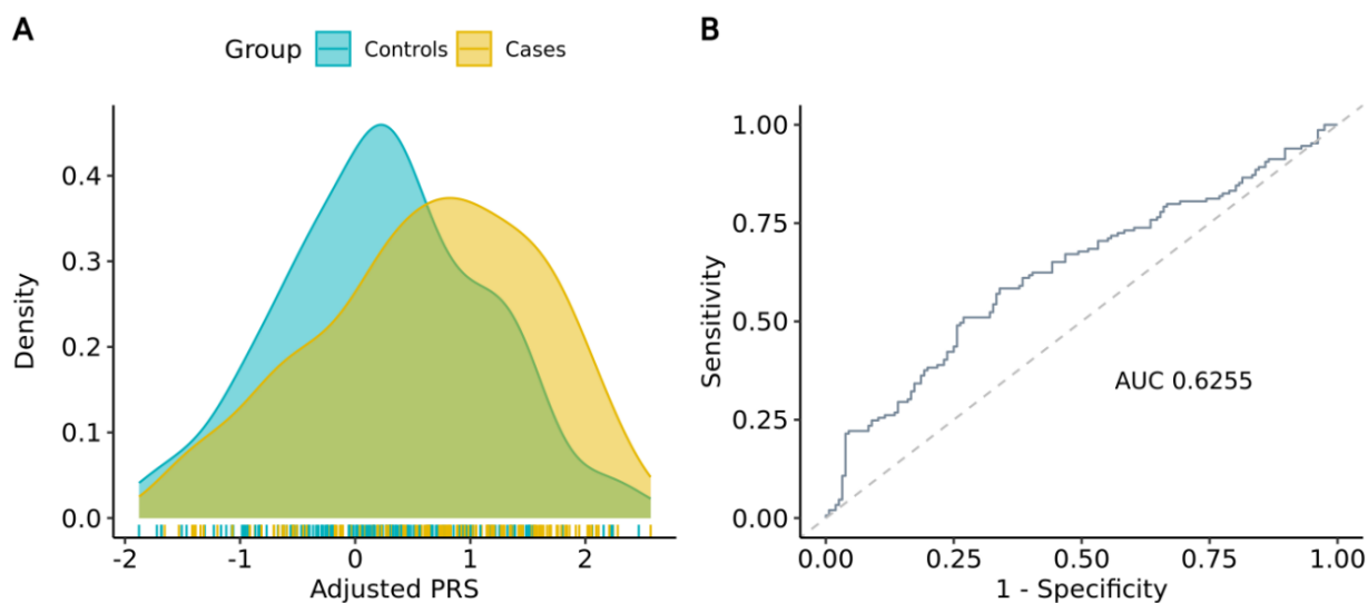
Supplementary Figure 1: Distribution curve and predictive accuracy of ancestry-adjusted PRS. (A) Distribution curve of adjusted PRS in cases vs. controls. Higher PRS were observed in the case group compared to the controls ( 0.63 \pm 0.97 vs. 0.24 \pm 0.88 ; p-value: 2.20 \times 10^{-3} ). (B) ROC curve for adjusted PRS. The observed AUC is 0.6255.
