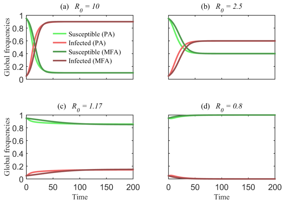
Fig. 2. The temporal dynamics of the global frequencies of susceptible ( P_S ) and infected ( P_I ) individuals under four scenarios of the R_0 value (10, 2.5, 1.17, and 0.8). The description, initial conditions, and parameters used are the same as in the caption of figure 1, and z = 100 .
