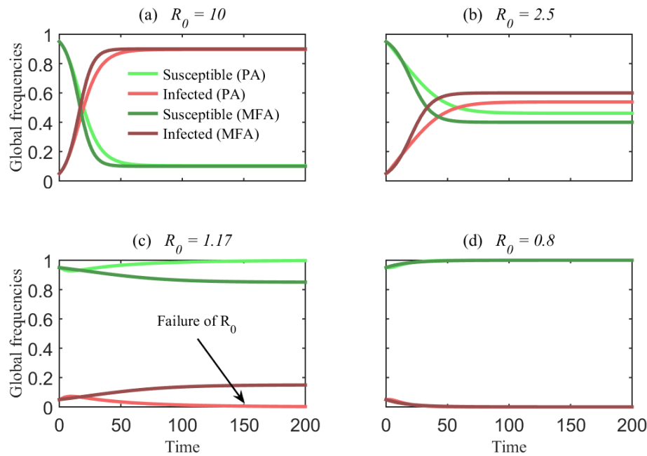
Fig. 1. The temporal dynamics of the global frequencies of susceptible ( P_S ) and infected ( P_I ) individuals under four scenarios of the R_0 value (10, 2.5, 1.17, and 0.8). The global frequencies of the pair-approximation (PA) model are represented by the bright-green and red curves, respectively, while the dark curves correspond to the mean-field approximation (MFA) model. The x-axis represents the simulation time, and the y-axis represents the global frequencies. The initial conditions: P_S(0) = 0.95 , P_I(0) = 1 - P_S(0) , P_{SI}(0) = 0.05 , P_{SS}(0) = 0.8 , and q_{IS}(0) = P_{SI}(0)/P_S(0) . Parameters used: \beta = 0.2 , R_0 = 10, 2.5, 1.17 , and 0.8 , \gamma = \beta/R_0 , and z = 4 .
