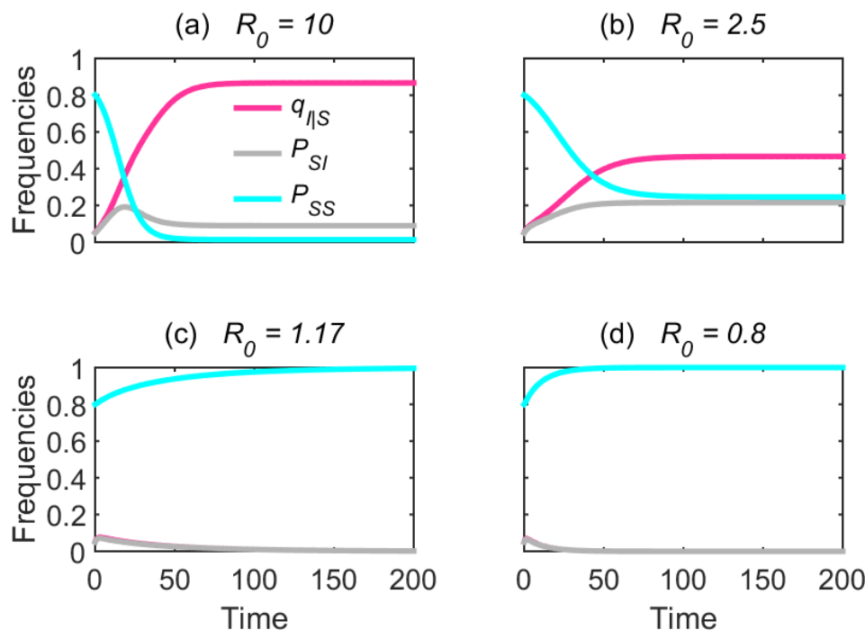
Fig. 4. The temporal dynamics of the average local frequency ( q_{II_S} , pink curve), neighbouring pairs of susceptible and infected individuals ( P_{SI} , grey curve), and neighbouring pairs of susceptible individuals ( P_{SS} , cyan curve) predicted by the pair-approximation model under four scenarios of the R_0 value (10, 2.5, 1.17, and 0.8). The x-axis represents the simulation time, and the y-axis represents the frequencies. The initial conditions: P_S(0) = 0.95 , P_I(0) = 1 - P_S(0) , P_{SI}(0) = 0.05 , P_{SS}(0) = 0.8 , and q_{II_S}(0) = P_{SI}(0)/P_S(0) . Parameters used: \beta = 0.2 , R_0 = 10, 2.5, 1.17, \text{ and } 0.8 , \gamma = \beta/R_0 , and z = 4 .
