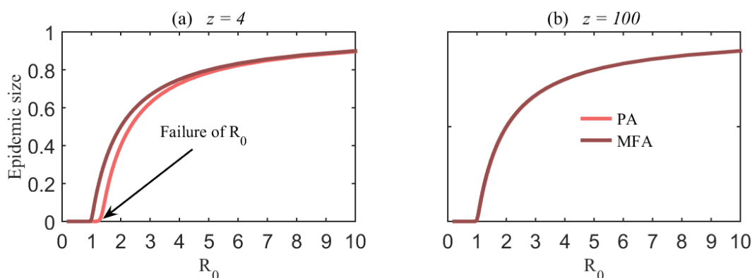
Fig. 3. The equilibrium dynamics of the epidemic size (y-axis) as a function the basic reproduction number R_0 (x-axis), predicted by the pair-approximation (PA) model (bright curve) and the mean-field approximation (MFA) model (dark curve). Initial conditions and parameter values are the same as in the caption of figure 1.
