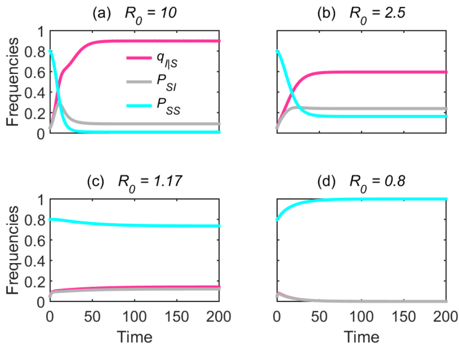
Fig. 5. The temporal dynamics of the average local frequency ( q_{I|S} , pink curve), neighbouring pairs of susceptible and infected individuals ( P_{SI} , grey curve), and neighbouring pairs of susceptible individuals ( P_{SS} , cyan curve) predicted by the pair-approximation model under four scenarios of the R_0 value (10, 2.5, 1.17, and 0.8). Initial conditions and parameter values are the same as in the caption of figure 4.
