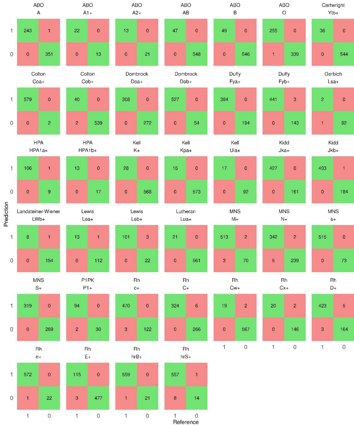
Figure 2. Confusion matrices of the Finnish models in the Finnish test data set.
