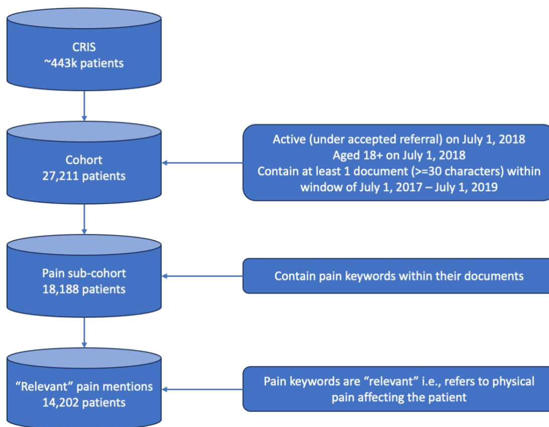
Figure 1. Data Extraction
