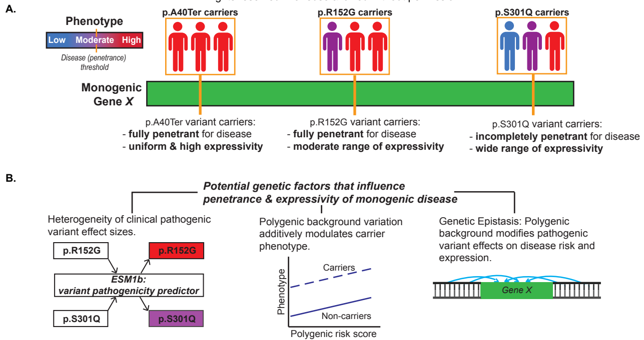
Figure 1: Outline of study. (A) We illustrate “penetrance” and “expressivity” with this cartoon. “Penetrance” is the fraction of carriers with disease and “expressivity” is the severity of the phenotype within carriers. (B) Our study focuses on three potential genetic factors that cause incomplete penetrance and variable expressivity: heterogeneous effect sizes of pathogenic variants, polygenic background, and genetic epistasis.
