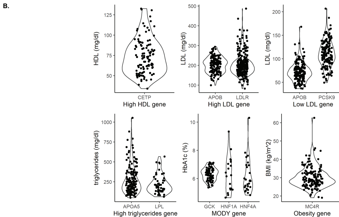
Figure 2: Carriers of pathogenic variants that affect cardiometabolic traits have incomplete penetrance and variable expressivity. (A) Penetrance thresholds were defined based on clinical definitions of disease. Relative to noncarriers (blue), carriers (pink) have higher penetrances (95% confidence intervals) for disease across all cardiometabolic phenotypes included in this study. Carriers also show incomplete penetrance of disease across all monogenic disorders. (B) Within pathogenic variant carriers, the distributions of phenotypes vary, consistent with variable expressivity.
