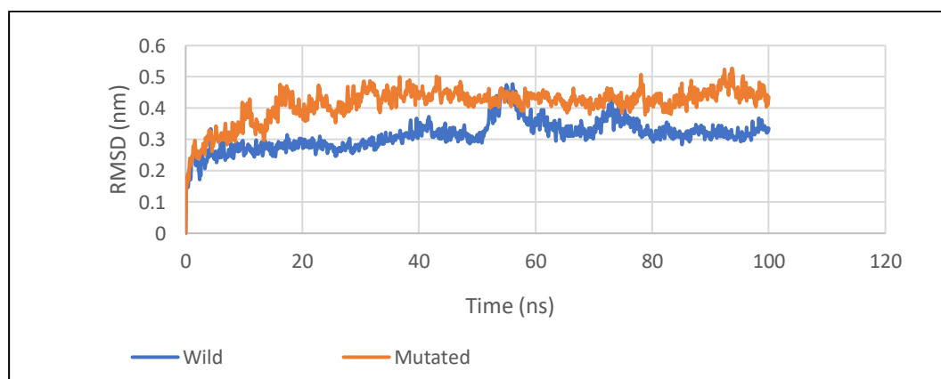
Fig:10 RMSD analysis of wild type ANXA11 and its variant (R452W) over time (ns)
