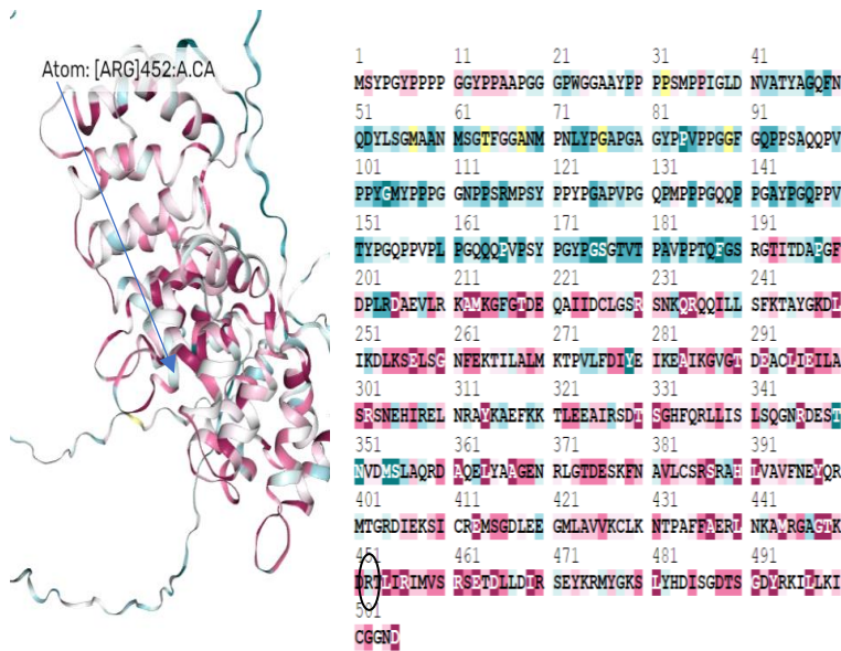
Fig: 3a Conservational analysis of ANXA11 wild. Conservation score= 2
