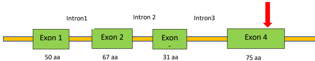
b. SIGMAR1 protein structure
