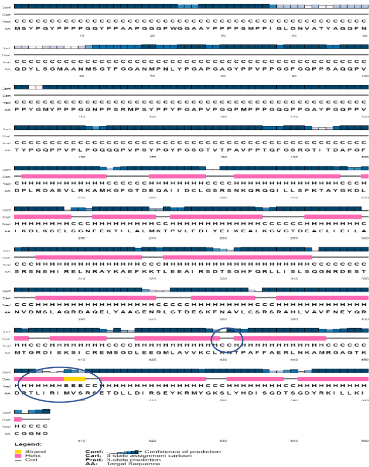
Fig:4 (a) Site of alterations shown in circle in the predicted secondary structure of a. ANXA11 wild type (b) ANXA11 R452W type by PSIPRED
