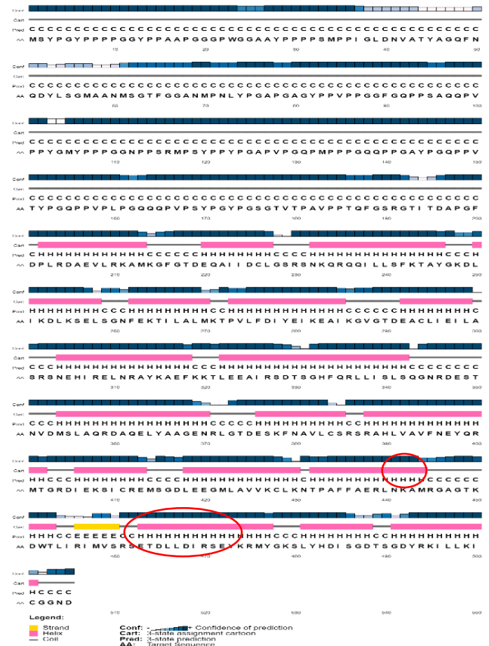
Fig:4 (a) Site of alterations shown in circle in the predicted secondary structure of a. ANXA11 wild type (b) ANXA11 R452W type by PSIPRED
