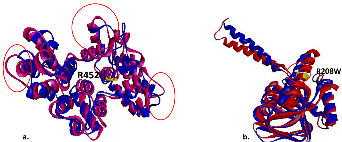
Fig: 9 Superimposed structure of wild and variant type of (a) ANXA11 and (b) SIGMAR . Blue denotes the wild type while Red denotes the mutated variant
