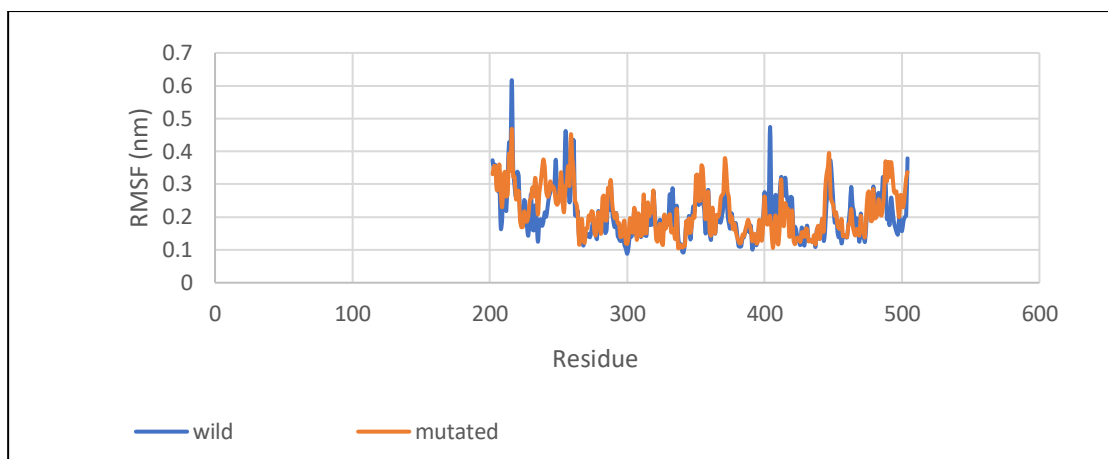
Fig:11 RMSF analysis of wild type ANXA11 and its variant (R452W)
