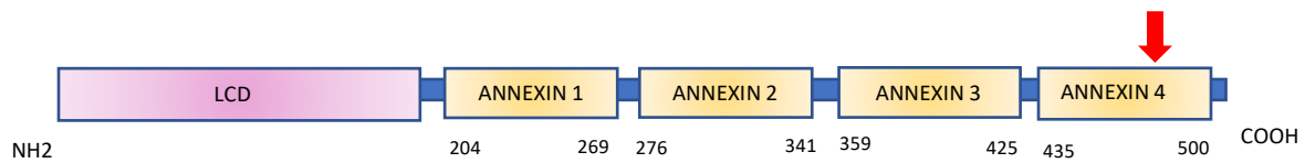
a. ANXA11 protein structure
