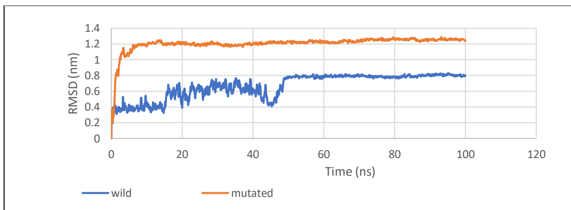
Fig:12 RMSD analysis of wild type SIGMARI and its variant (R208W) over time (ns)
