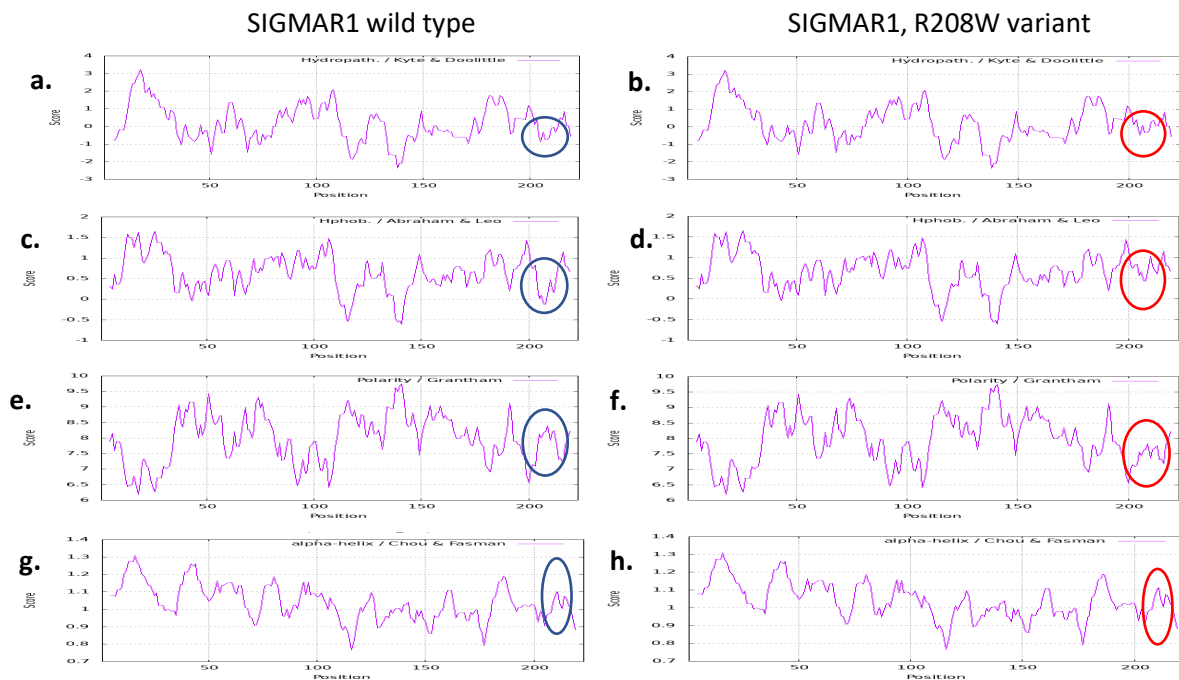
Fig 7: Physicochemical properties of SIGMAR1 wild vs R208W variant. (a,b) denotes increased hydropathicity of R208W compared to its wild type. (c,d) denotes increased hydrophobicity of R208W compared to its wild type. (e,f) denotes lower polarity of R208W compared to its wild type. (g,h) denotes slight increase in alpha helix of R208W compared to its wild type. The x-axis represents the position of the amino acids while the y-axis represents the score in a default window size of 9
