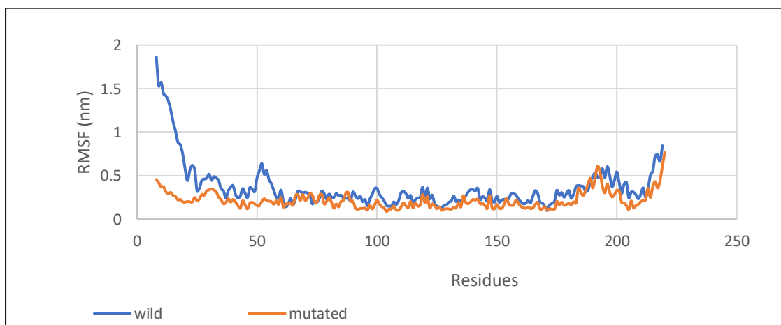
Fig:13 RMSF analysis of wild type SIGMARI and its variant (R208W)
