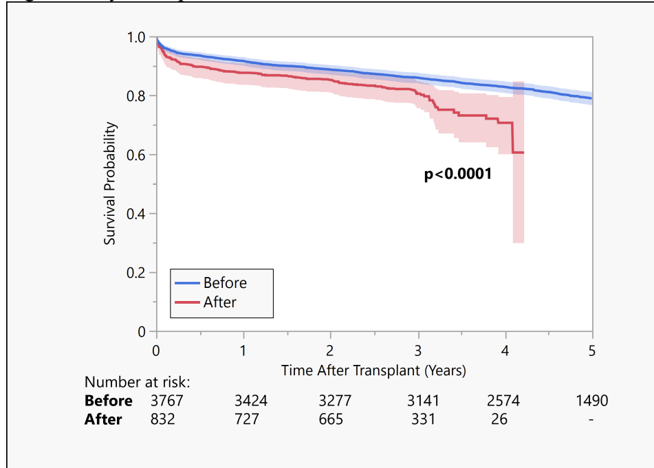
Figure 1. 5-year Kaplan-Meier Survival Curve for Before versus After Score Change
