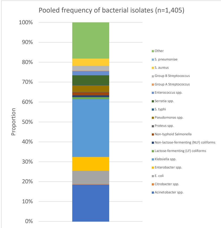
Figure 3. Pooled frequency of positive bacterial isolates
