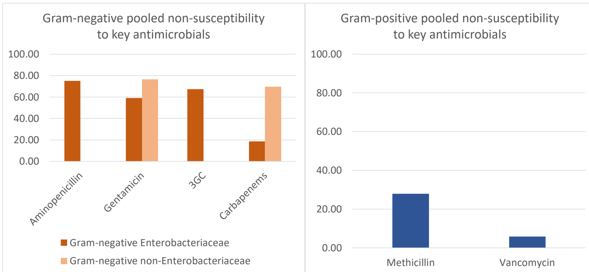
Figure 4. Pooled non-susceptibility to key antimicrobials for a) Gram-negative pathogens and b) Gram-positive pathogens
