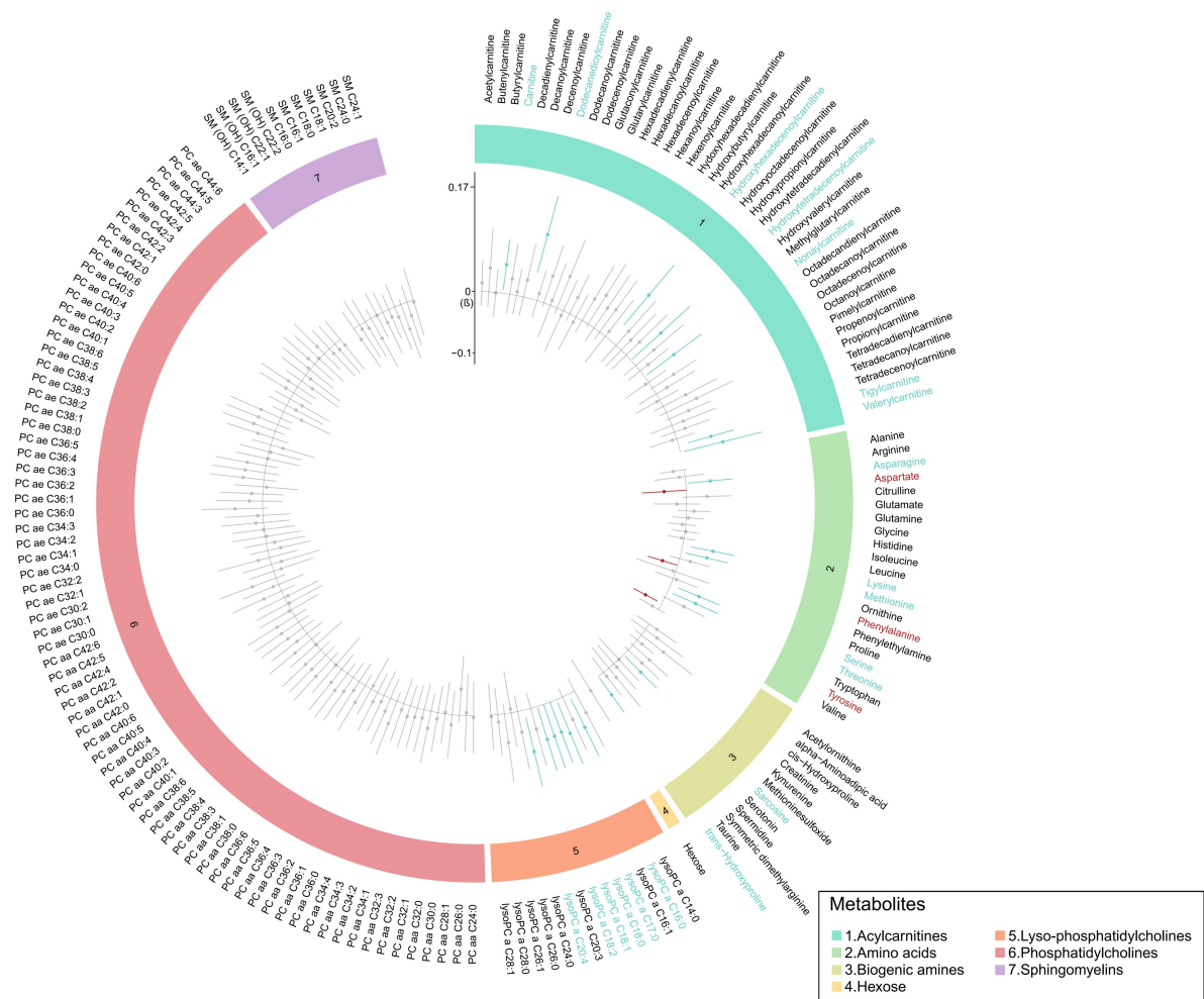
676 Fig 3. Circos plot depicting the causal effect estimates of puberty timing on all 174 677 plasma metabolites. The legend located at the lower section of the figure provides a visual 678 representation of distinct subclasses of plasma metabolites. The presence of metabolites 679 highlighted with the color blue indicates a positive causal effect of puberty timing on the 680 concentration of plasma metabolites. Specifically, each year later in puberty timing is 681 associated with higher levels of metabolites. In contrast, the identification of metabolites 682 highlighted with the color red suggests a negative causal effect of puberty timing on the 683 concentration of plasma metabolites, that is each year later in puberty timing is associated 684 with lower levels of metabolites. The presence of metabolites that had been designated as 685 black indicates that there is insufficient evidence to establish a causal relationship. The
