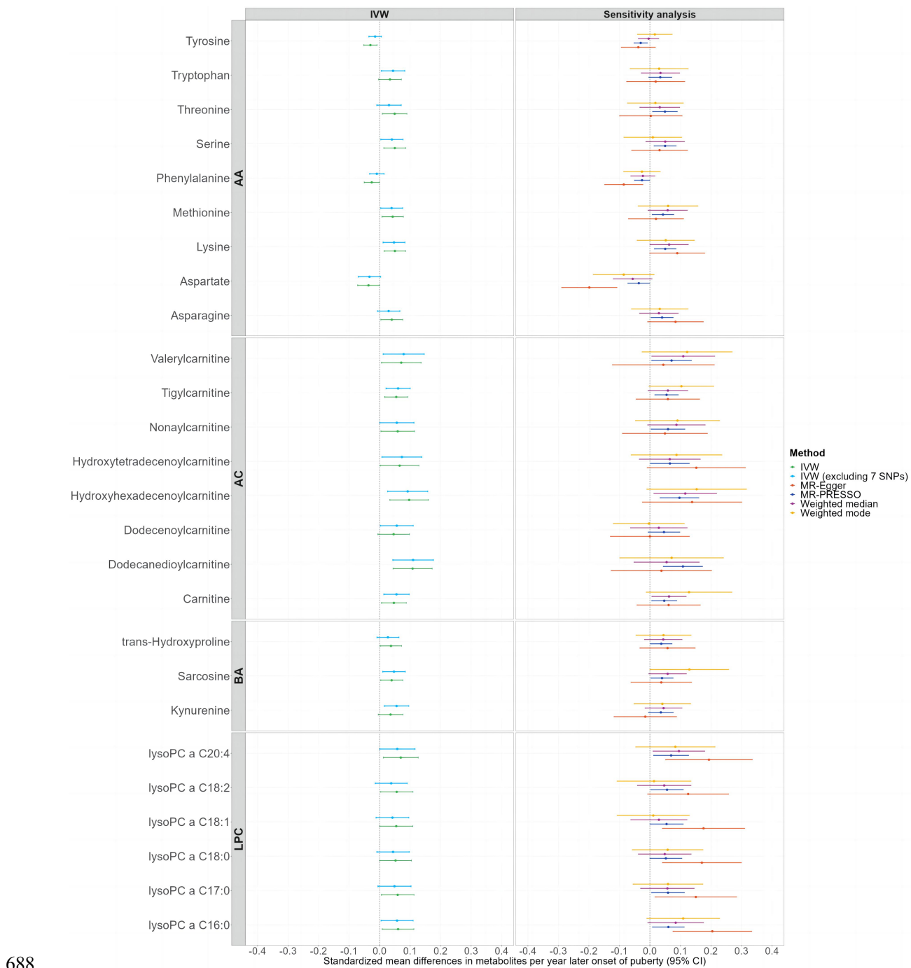
689 Fig 4. Forest plots showing the causal effect estimates of puberty timing on plasma 690 metabolites. The legend located on the right side of the forest plot indicates different analysis 691 approaches. Plasma metabolites reaching nominal significance ( P < 0.05 ) were shown 692 according to the results of IVW (inverse-variance weighted). The results presented on the left
