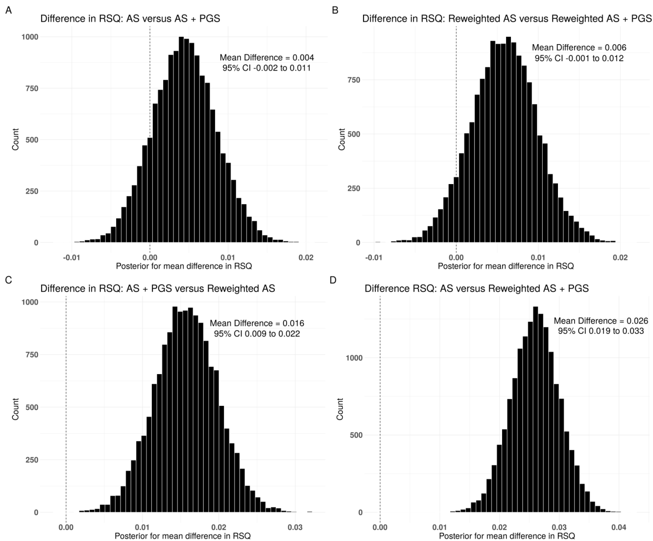
497 Figure 1. Between-model comparison of difference in explanation of variance (RSQ).
