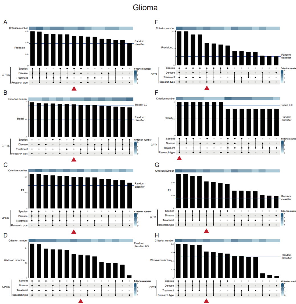
Figure 3 Best combination of single-prompts was identified by evaluating the performance of all combinations of single-prompts from glioma meta-analysis
