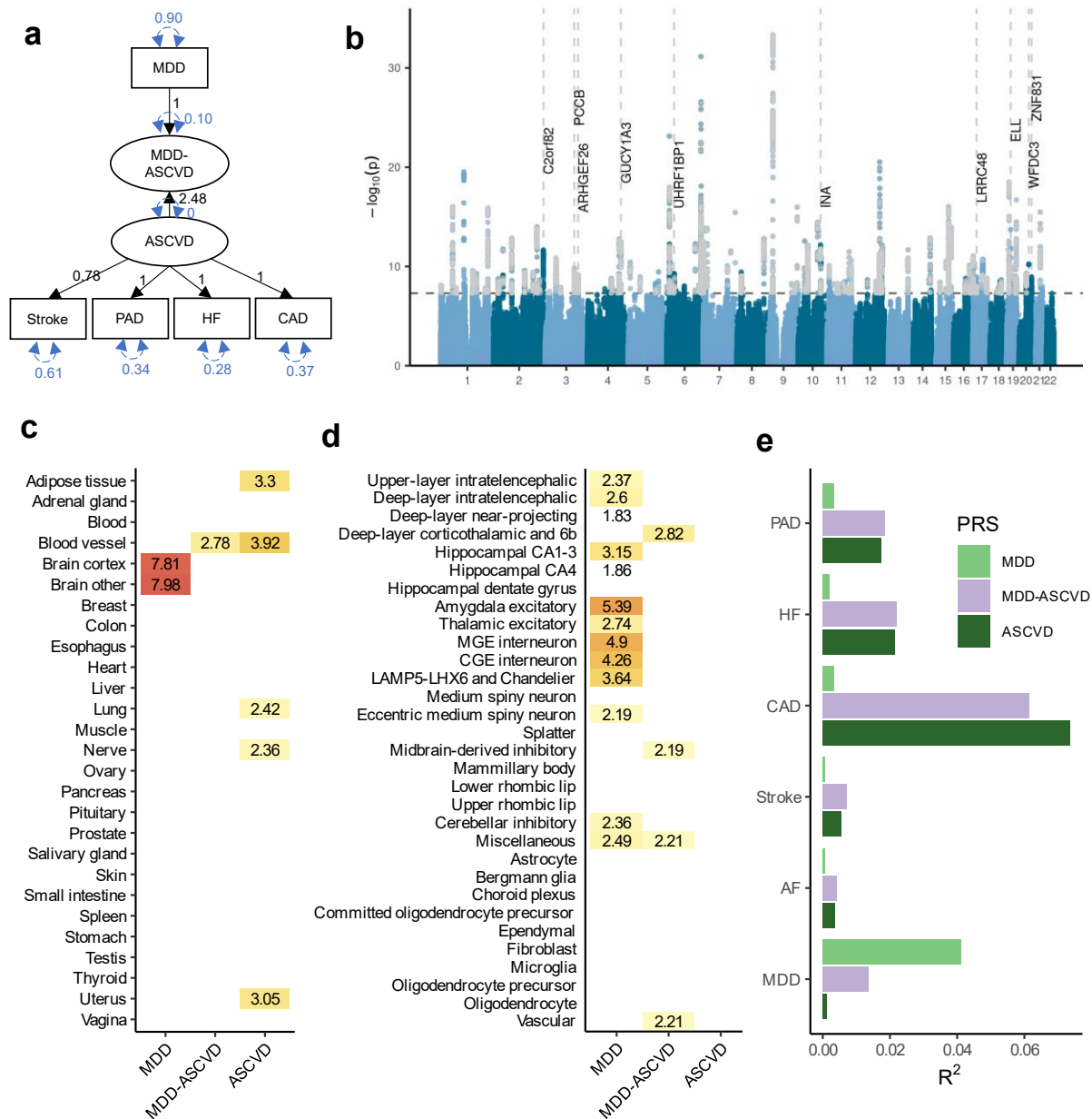
Figure 3. Shared genetic liability factor for MDD-ASCVD. (a) Latent factor model as specified in Genomic SEM with the ‘observed’ variables in rectangles and the latent variables in circles. Factor loadings (standardized on the latent factors) are given in black and variances in blue. Sample sizes for underlying GWAS summary statistics are reported in Supplementary Table 1 (b) Latent MDD-ASCVD factor GWAS results. The x-axis shows genomic position, and the y-axis shows statistical significance as -\log_{10}(P) . Genome-wide significant SNPs that were filtered out because of significant heterogeneity Q_{SNP} are displayed in grey. The top 10 eQTL genes are displayed with dashed vertical lines indicating their position. (c) Enrichment results in GTEX tissues for the latent MDD-ASCVD factor, with latent ASCVD (without MDD) and MDD-only as comparison. (d) Enrichment results for the latent MDD-ASCVD factor, latent ASCVD, and MDD-only in brain cell types. (e) Proportion of variance explained in MDD and CVD phenotypes in the UKB (defined using ICD-codes listed in Supplementary Table 14) by each of 3 PRSs for the latent MDD-ASCVD factor, latent ASCVD, or MDD-only. c, d Enrichment is measured using significance testing in a two-sided t-test displayed as -\log_{10}(P) . Only tissues with a significant association ( P_{FDR} < 0.05 ) are shown. Multiple testing was performed over tested tissues/cell-types.
