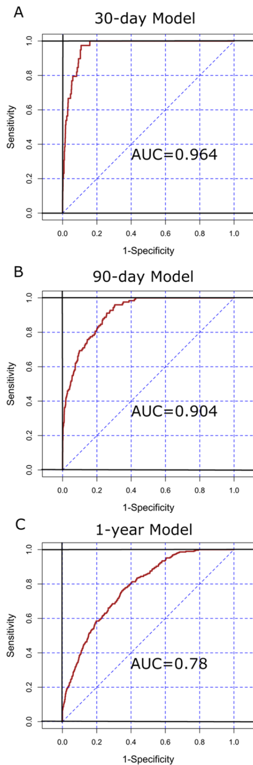
546 Figure 3. Area Under the Receiver Operating Characteristic Curve using 547 Interaction terms. 548
