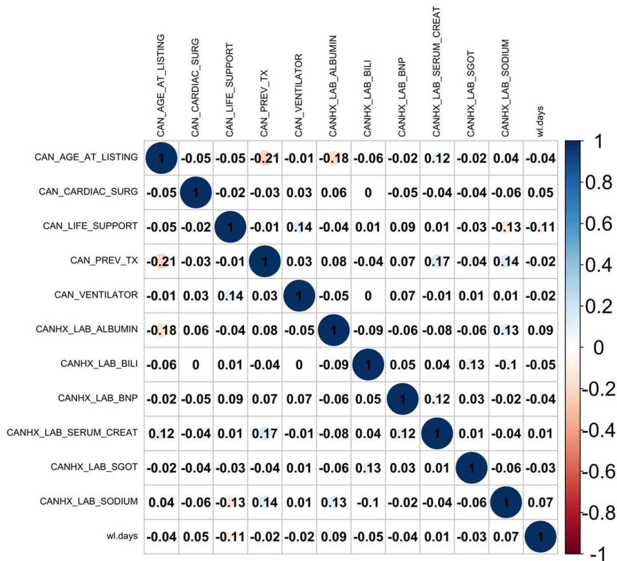
541 Figure 1. Correlation Heatmap of Independent Variables.
