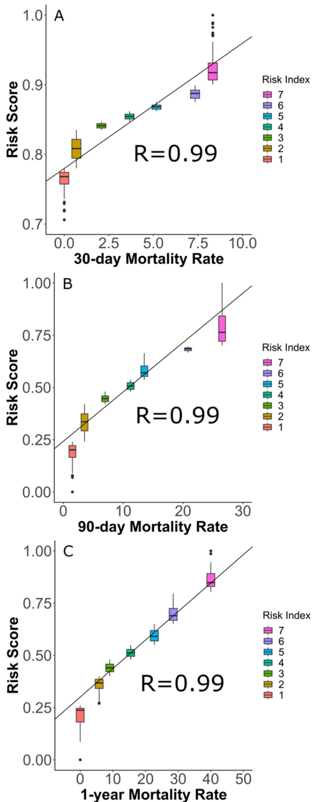
543 Figure 2. Calibration Plots for 30-day, 90-day, and 1-year Models. 544
