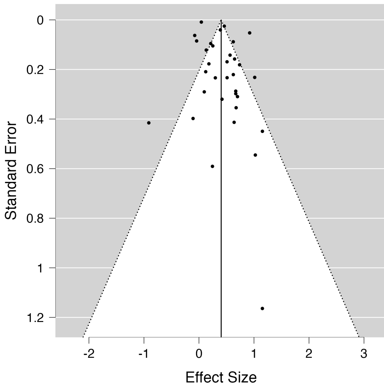
Figure 3: Funnel Plot
