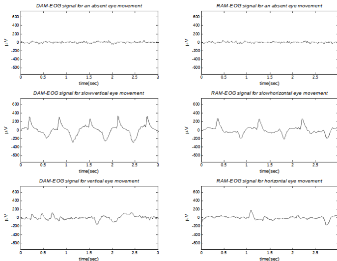
Figure 3: Typical EOG signals recorded for three situations described in the text. Large changes occurred in EOG signals when the subject moves eyes slightly. Even when subject moves eyes slowly, changes in EOG can be easily identified. The above graphs are drawn for the data recorded from subject S1.
