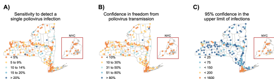
170 171 Figure 1: The sensitivity of wastewater treatment plants in New York State to a) detect a single poliovirus infection, b) provide 172 confidence in the freedom from poliovirus transmission with three consecutive non-detections, and c) provide 95% confidence in 173 the upper limit of the number of poliovirus infections with three consecutive non-detections.
