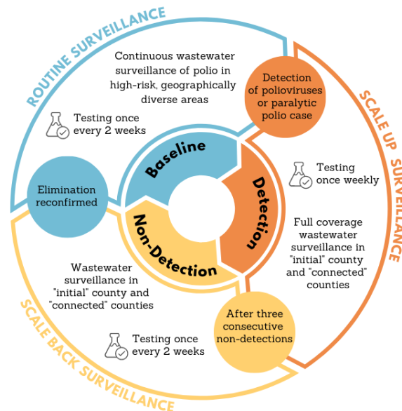
264 Figure 3: Conceptual framework to guide the frequency and scale of testing wastewater for poliovirus. 265 Baseline prospective surveillance regularly tests wastewater from communities vulnerable to polio 266 outbreaks. Detection prompts a scale-up in surveillance, increasing both the spatial coverage and 267 temporal frequency. Consecutive non-detections prompt scaling back in surveillance, reducing the 268 temporal frequency. Once elimination is confirmed the system returns to baseline prospective 269 surveillance.
