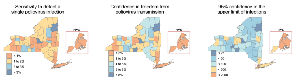
179 180 Figure 2: The sensitivity of New York State’s wastewater surveillance to identify at the county level a) a single poliovirus 181 infection, b) confidence in the freedom from poliovirus transmission with three consecutive non-detections, and c) an upper limit 182 of the number of poliovirus infections given three consecutive non-detections.
