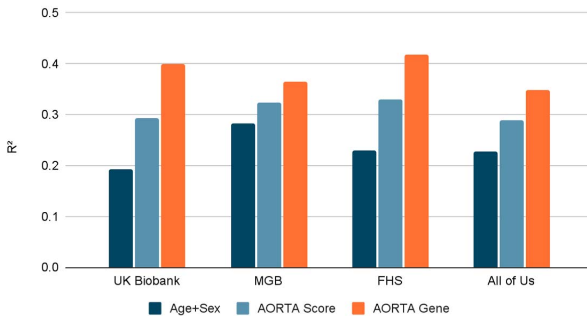
Figure 3: Variance in aortic diameter explained by the models
