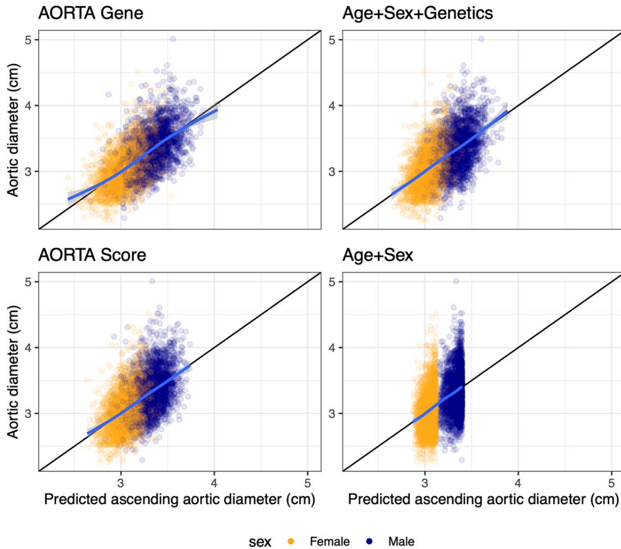
Figure 2: Score calibration curves in the UK Biobank validation set
