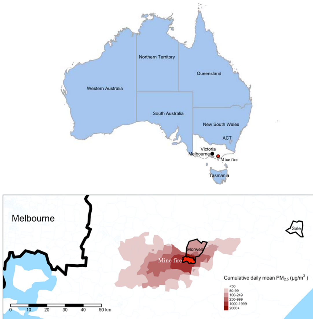
Figure 1. Maps of Australia illustrating location of the coalmine and distributions of fire related-PM 2.5 (February to March 2014) in the surrounding areas, highlighting exposure site Morwell and control site Sale
