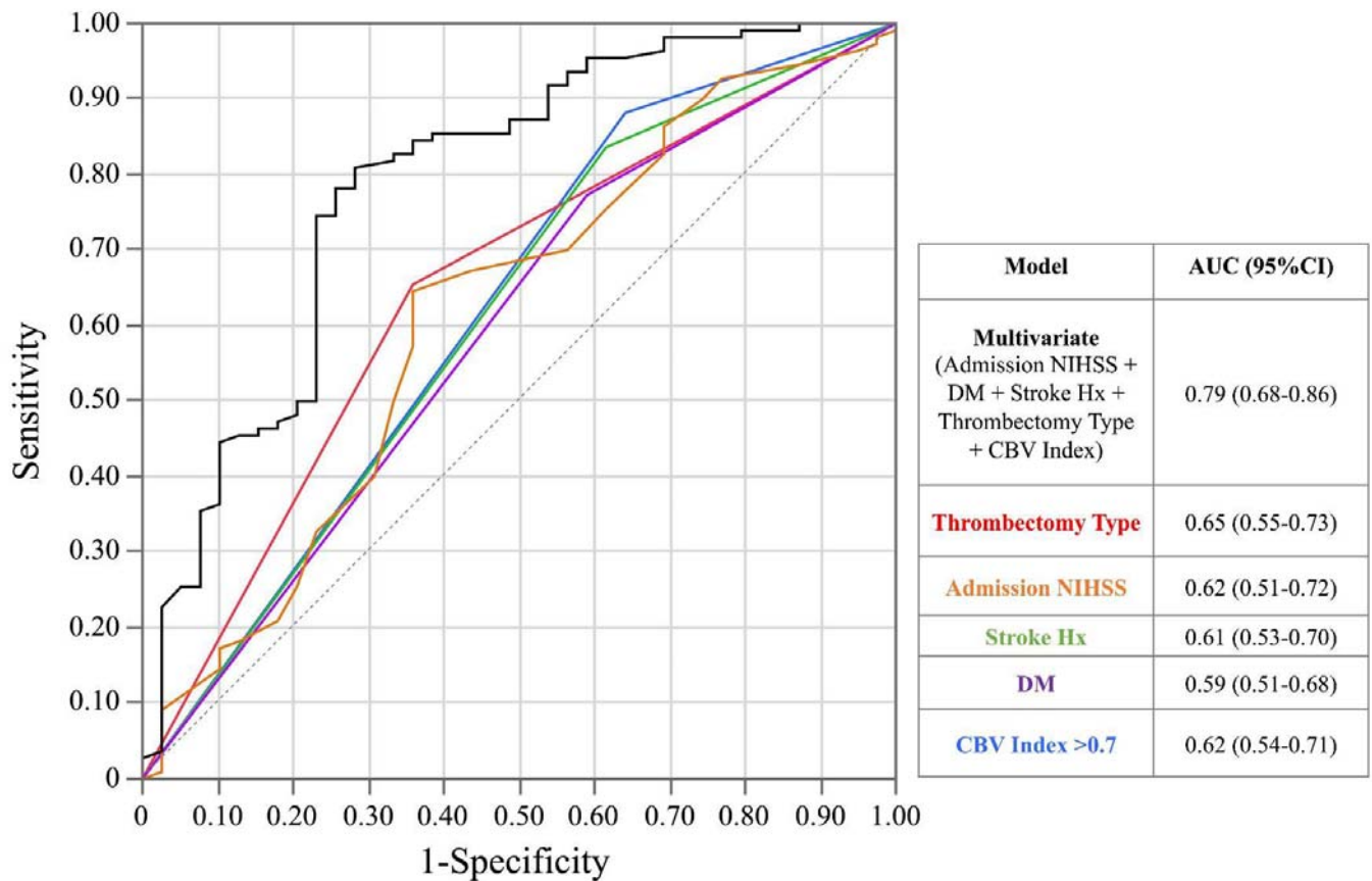
Figure 1: Receiver operator characteristics curve with area under the curve for dichotomized CBV index (>0.7), admission NIHSS, diabetes mellitus, prior stroke history, and aspiration thrombectomy as univariate factors and the combined multivariate model for outcome of mTICI 2C/3 versus 2B. Abbreviations: CBV = cerebral blood volume, NIHSS = National Institutes of Health Stroke Scale, mTICI = modified thrombolysis in cerebral infarction score, AUC = area under the curve, CI = confidence interval, DM = diabetes mellitus, Stroke Hx = stroke history.
