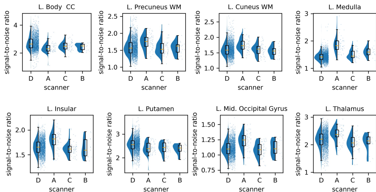
Fig. 8 Signal-to-noise ratio (SNR) of the FA images across 8 Eve type-1 atlas-defined ROIs, including white matter (WM) regions (body of the corpus callosum, precuneus WM, cuneus WM), gray matter regions (insular, putamen, middle occipital gyrus, thalamus), and mixed regions (medulla), in 4 different scanners of BLSA (where scanner A is the 1.5 Tesla Philips Intera scanner, and scanners B/C/D are the 3 Tesla Philips Achieva scanners). “L.” stands for the left hemisphere of the brain.
