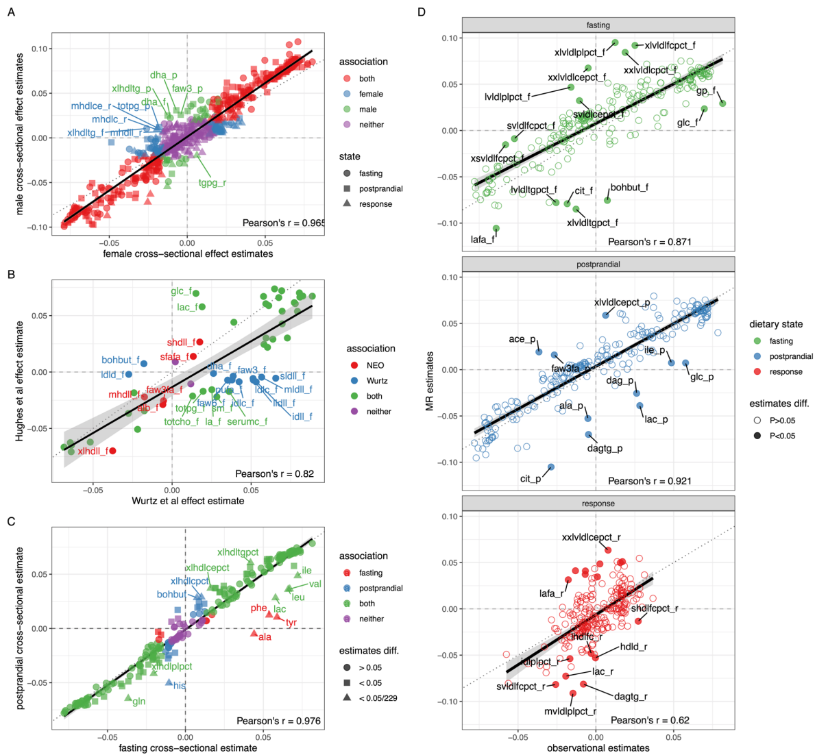
Figure 3: Scatter plots. In all plots the solid black line is a best fit regression line, the dotted black line is an equivalency line (intercept = 0, slope = 1), the dashed vertical and horizontal line indicate the zero values, and a Pearson's correlation coefficient is in the bottom right corner. (A) Scatter plot of
