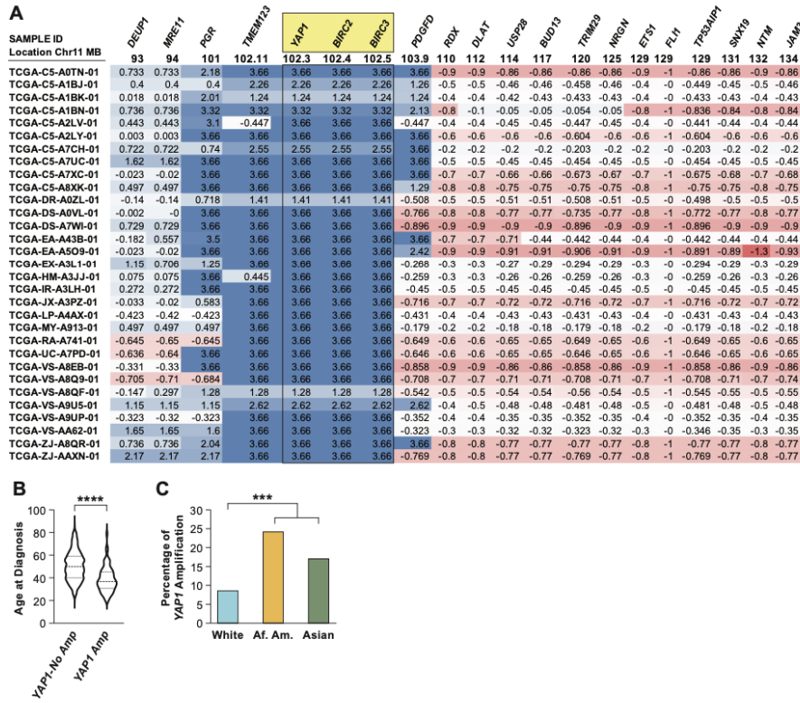
Figure 8. Analysis of YAP1 gene amplification in 31 cervical tumors. A. Copy number data for genes centromeric and telomeric to YAP1 in all TCGA cervical tumors with Log 2 copy number values for YAP1 >1. The location of the YAP1 , BIRC2 and BIRC3 genes are highlighted. The location of each gene in MB is given below the gene symbol. B. Comparison of the age of diagnosis between women with YAP1 -amplified and unamplified tumors C. Self-identified race of cervical cancer patients with and without YAP1 amplification. Data from TCGA, MSKCC metastatic cancer, and AACR GENIE cohort were obtained from cbiportal ( https://www.cbiportal.org ) (Cerami et al., 2012; Gao et al., 2013).
