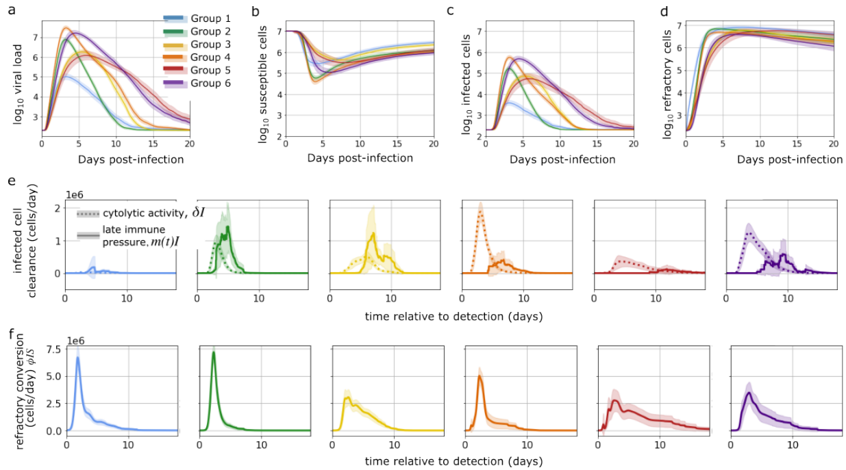
Figure 4: Mechanistic differences between dynamic groups. Panels (a-d) show the mean viral load and cell populations in the mechanistic model for each group over time with 95% confidence interval shaded. The quantities are (a) log viral load, \log_{10}(V) , (b) number of susceptible cells, \log_{10}(S) , (c) number of active infected cells, \log_{10}(I) and (d) the number of cells refractory to infection \log_{10}(R) . Next, we plot the mean and standard deviation of immune pressures over time for each dynamic group. Panel (e) shows the infected cell clearance due to both constant cytolytic activity and delayed immune pressure. Panel (f) shows the conversion of susceptible cells to a refractory state.
