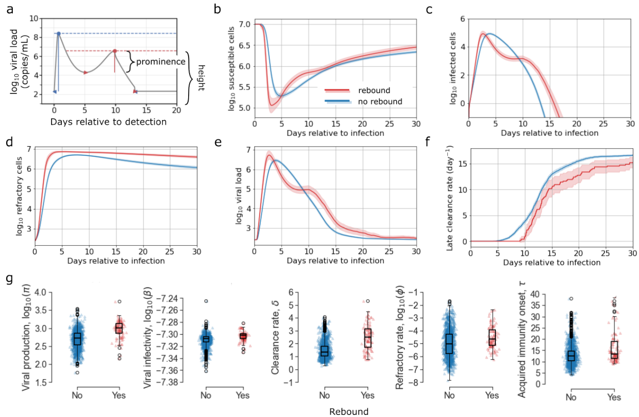
Figure 6: Model fitting to viral rebound in the NBA cohort. (a) We classified infections as examples of viral rebound if there are at least two peaks in the model simulation with height of 3 logs and prominence of 0.5 log. Mean (b) number of susceptible cells, (c) number of active infected cells, (d) number of target cells that are refractory, (e) viral load, and (f) rate of late clearance as predicted by our mathematical model for rebound vs. non-rebound cases in red and blue respectively. 95% confidence interval shaded. (g) Distribution of individual parameter estimates for the rebound vs. non-rebound cases. Only those for which the mean differs significantly are displayed ( p_{adjusted} < .05 for Mann-Whitney U test).
