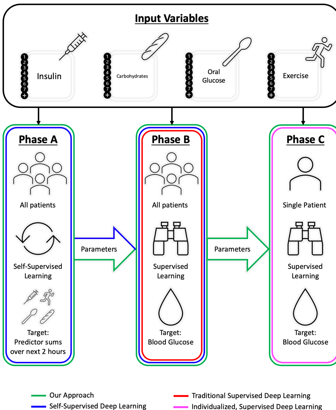
Fig 2. The Training Phases of our Novel Approach: First we perform a phase of self-supervised learning on the abundant predictor data of all patients. During this phase, the task is to predict the four sums of our predictors over the next 24 entries. This is followed by a phase of traditional supervised learning on all patient’s blood glucose labels. Finally, we leverage individualization with a final training phase that fine-tunes on the individual patient’s blood glucose labels. Other approaches tested are also highlighted.
