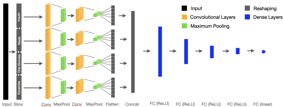
Fig 1. Model Architecture for All Experiments: We first feed the four time series predictors through a series of two 1D convolutional layers with batch normalization and dropout. We then concatenate the output from this and use linear layers to arrive at a single output.
