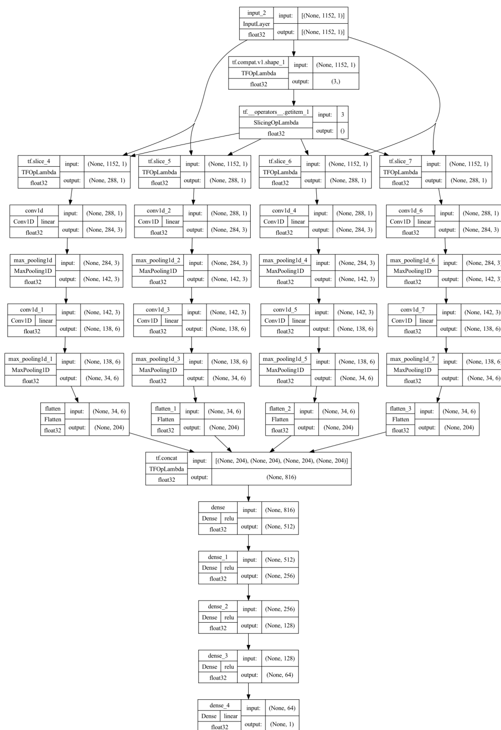
Fig 6. Fully detailed model architecture including layer sizes. Included for completeness.
