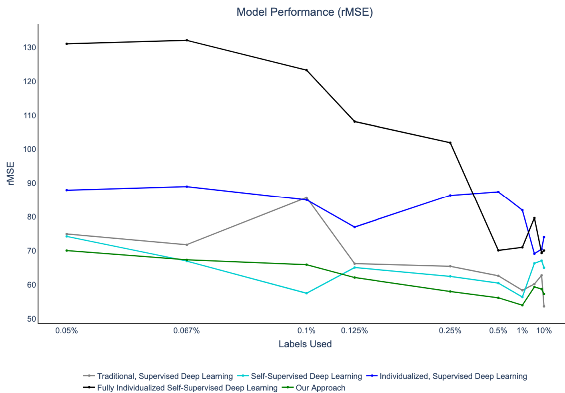
Fig 4. Model Performance under different training approaches in rMSE: Test rMSE of baseline approaches and our approach for different levels of data label availability. Included for interpretability.
