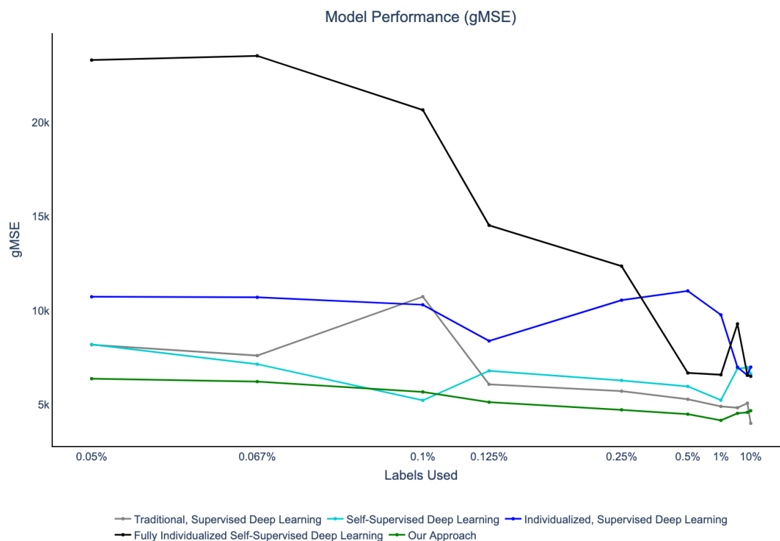
Fig 3. Model Performance under different training approaches in gMSE: Test gMSE of baseline approaches and our approach for different levels of data label availability. (see Table 1).
